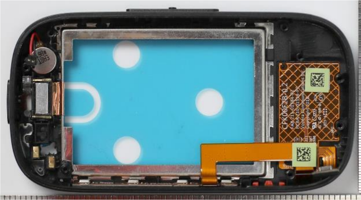
Front cover without LCD display
