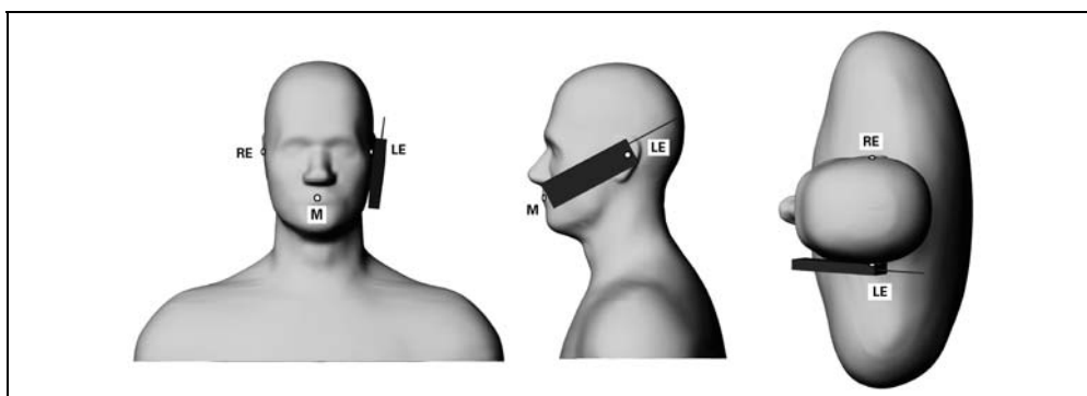
Figure 1. Position 1, "cheek" or "touch" position. The reference points for the right ear (RE), left ear (LE) and mouth (M), which define the reference plane for device positioning, are indicated (Shoulders are shown for illustration only).
