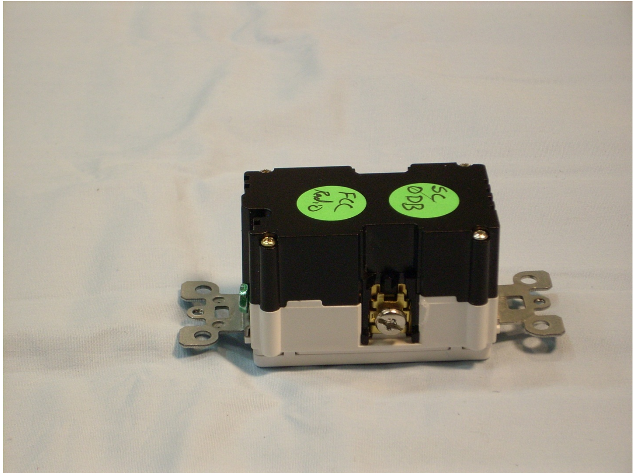
Back/Side View of the EUT Outside Metal Wallbox
