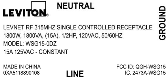
Figure 1. WSG15-0DZ (Same for IC and FCC)
