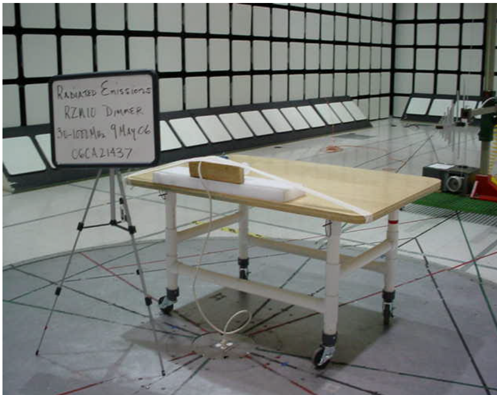
Model RZM10 – Rear View 30-1000MHz
