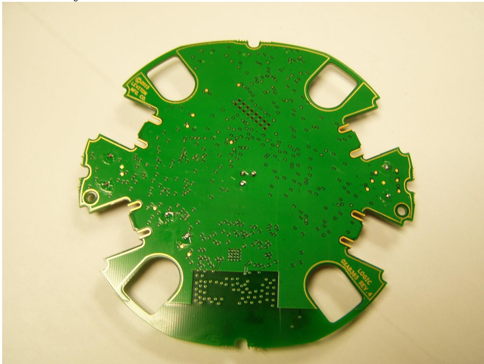
Rear view Provolt logic board with radio
