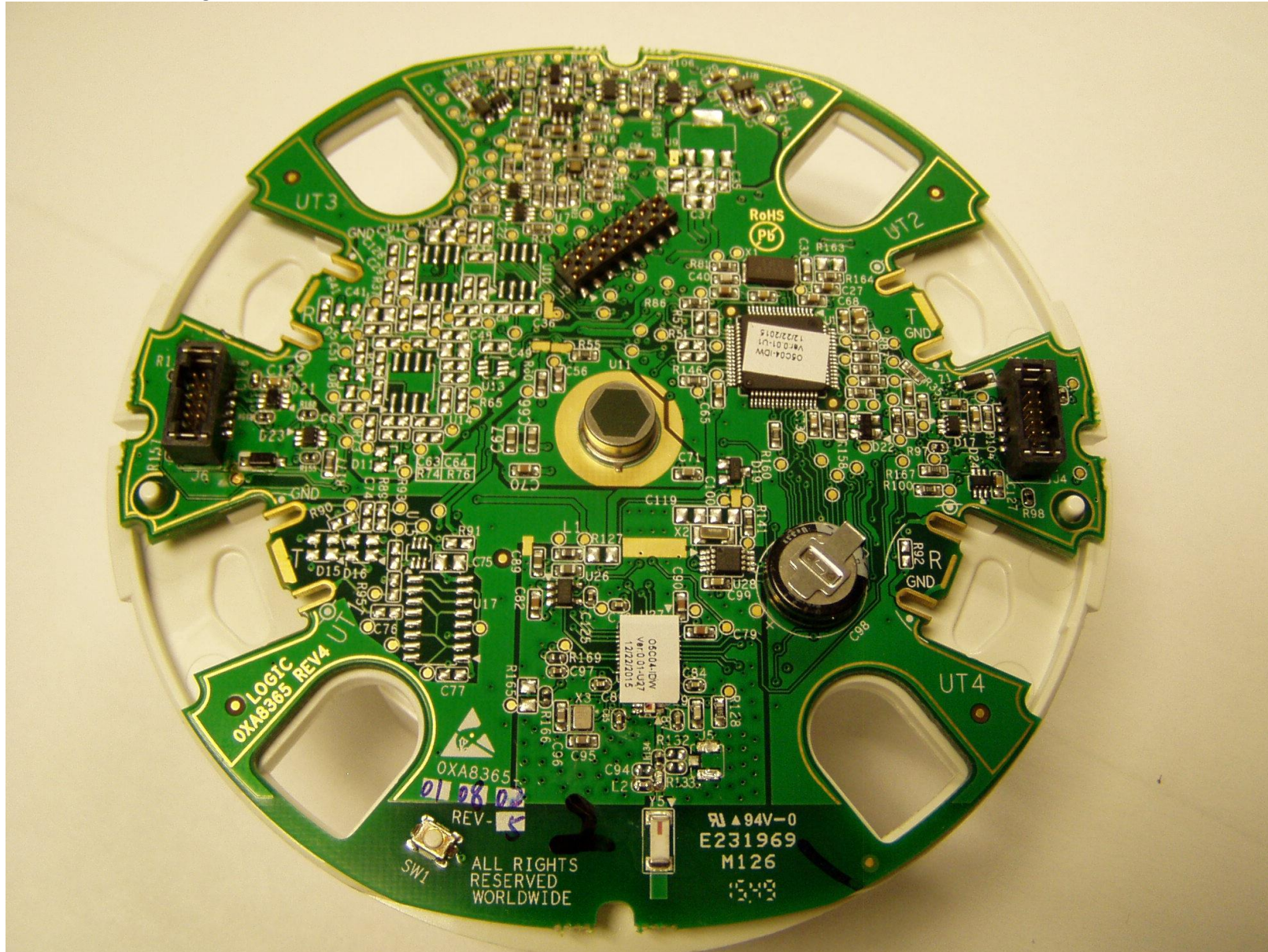
Front view Provolt logic board with radio
