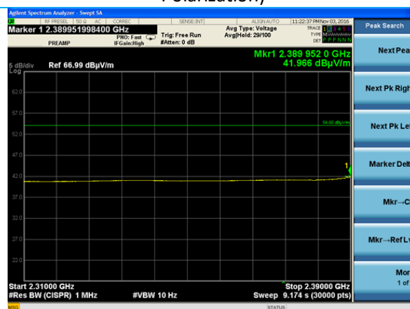
Lower Band Edge (Average, Low Channel)
