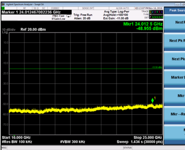
10000-25000 MHz (11)
