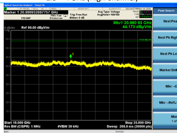
18 - 25 GHz (High Channel, Horizontal Polarization)
