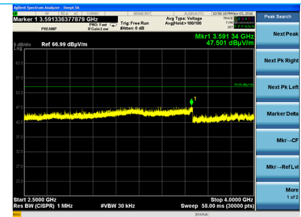
2.5 - 4 GHz (High Channel)
