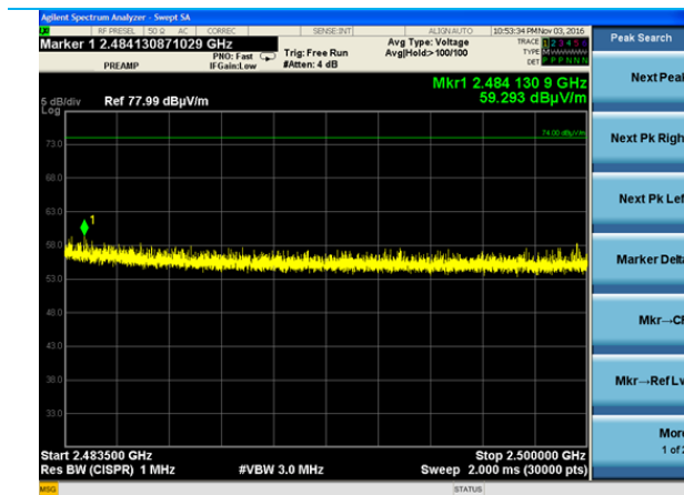
Upper Band Edge (Peak, High Channel)
