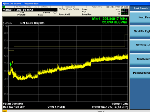
200 – 1000 MHz (Low Channel, Vertical Polarization)
