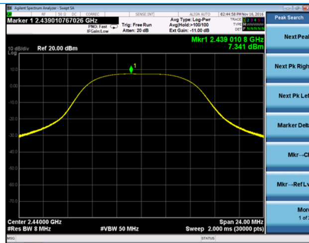
Channel 18 Pout
