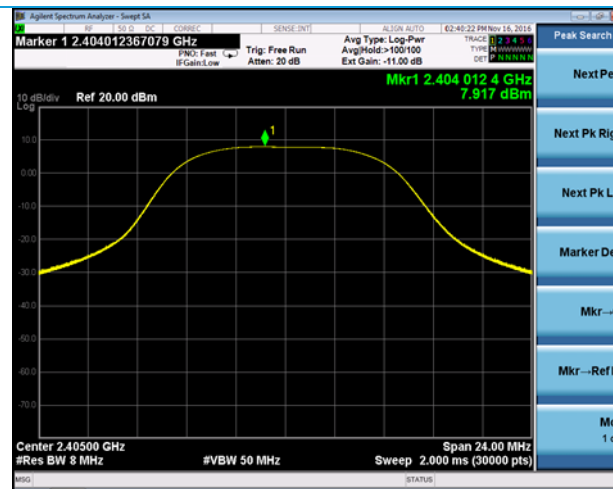
Channel 11 Pout
