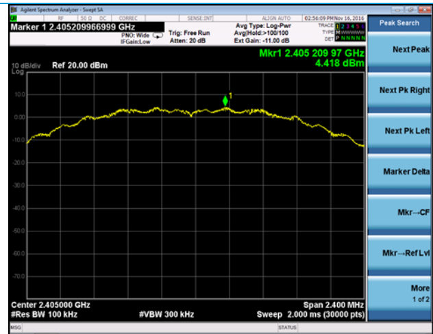
Channel 11 (Limit = -15.582 dBm)
