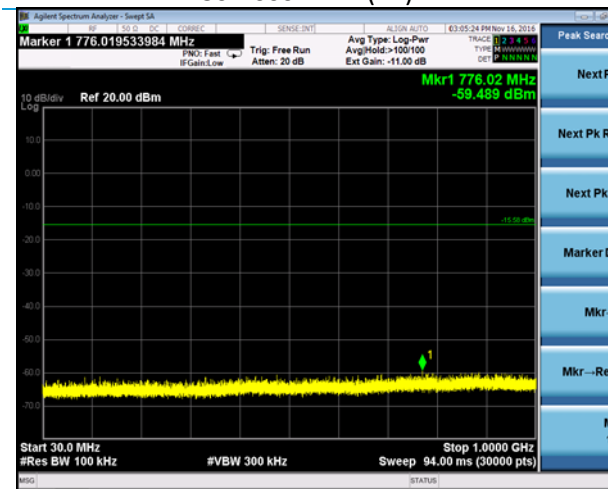
30-1000 MHz (18)
