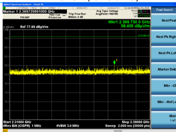
Lower Band Edge (Peak, Low Channel)
