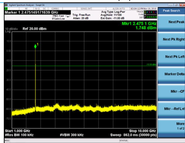
1000-10000 MHz (25)
