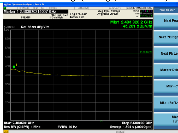
Upper Band Edge (Average, High Channel)
