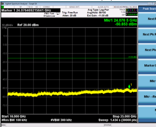
10000-25000 MHz (25)
