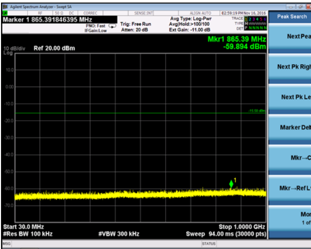
30-1000 MHz (26)
