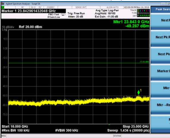
10000-25000 MHz (18)
