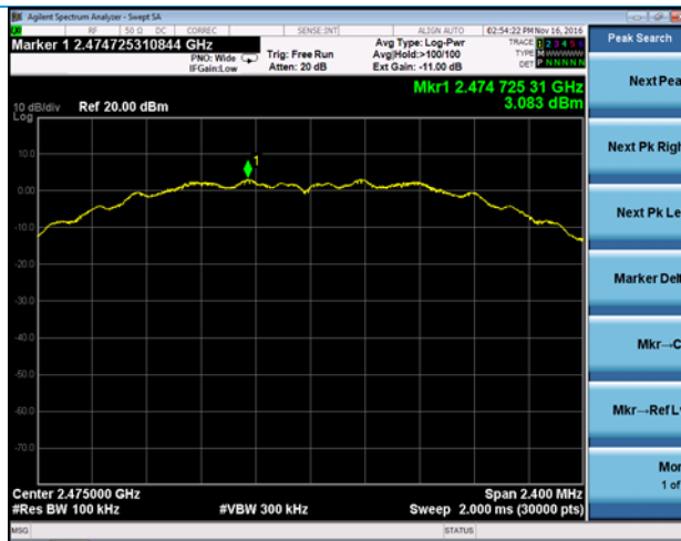
Channel 25
