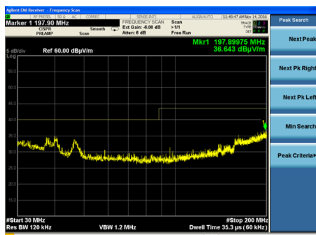
30 – 200 MHz (Low Channel, Vertical Polarization)
