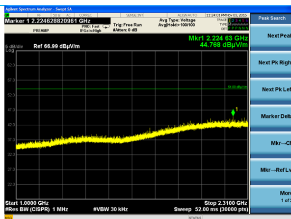
1 – 2.31 GHz (Low Channel)
