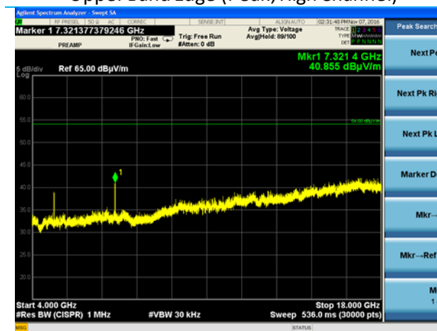
4 - 18 GHz (High Channel, Horizontal Polarization)
