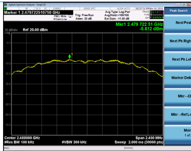
Channel 26
