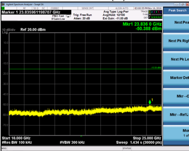
10000-25000 MHz (26)
