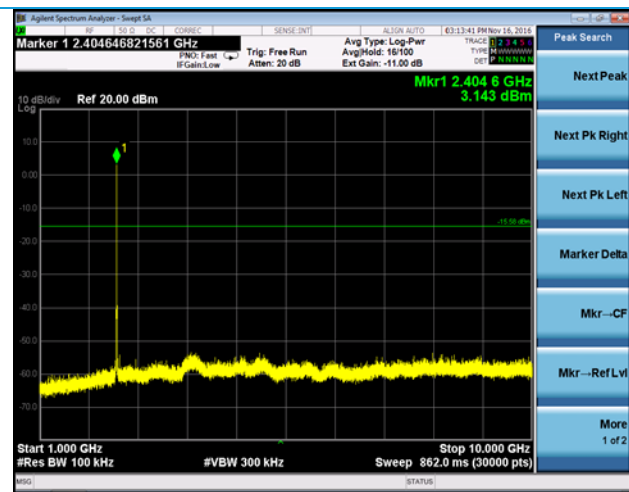
1000-10000 MHz (11)
