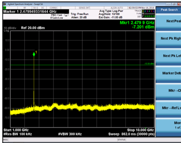
1000-10000 MHz (26)
