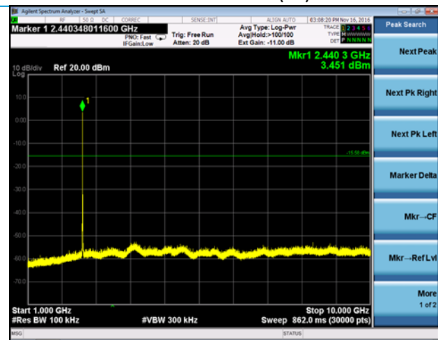
1000-10000 MHz (18)
