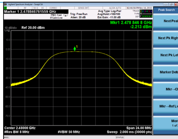
Channel 26 Pout
