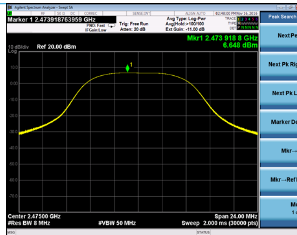
Channel 25 Pout
