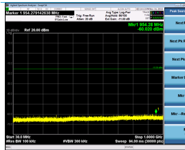
30-1000 MHz (11)
