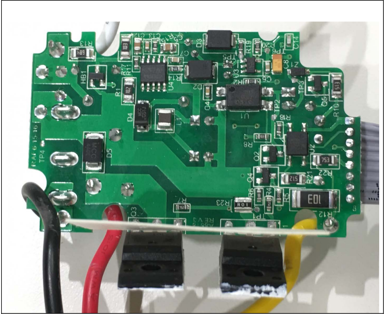
DDE06 AC Mains Board Bottom
