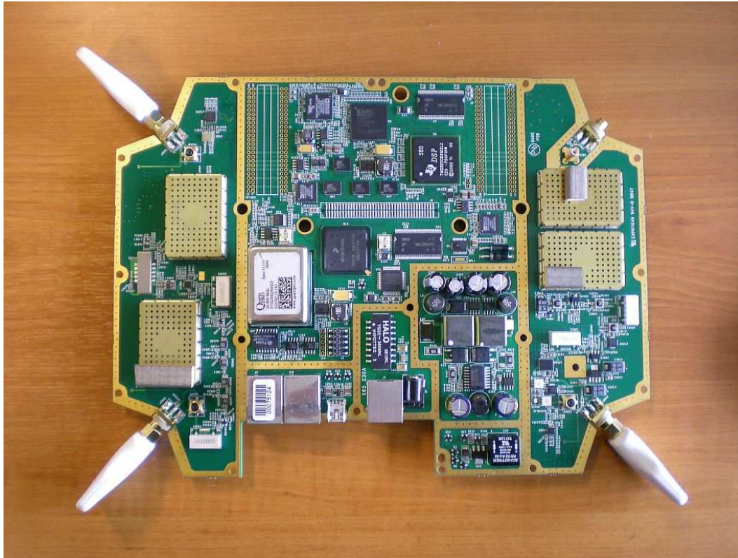
165H-PCB(Top)
