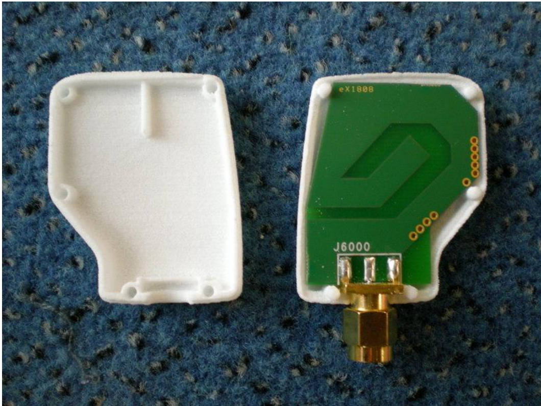
165D-Antenna
