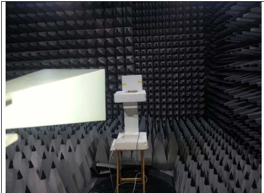
Fig 4 Test setup 18-22GHz Rad Emission
