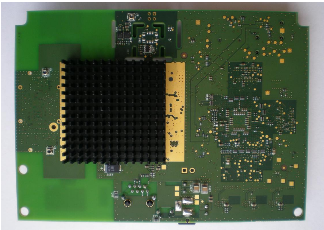
Bottom View
