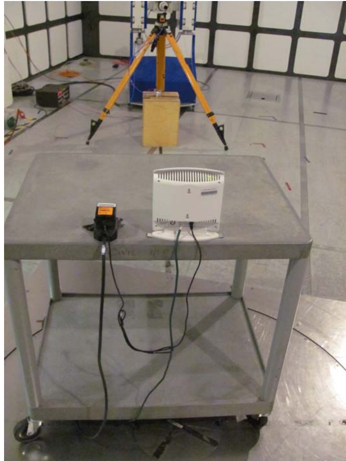
Radiated Emissions 18GHz-20GHz
