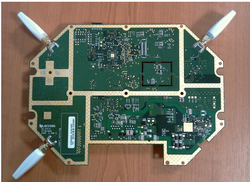
239B – PCB (Bottom)
