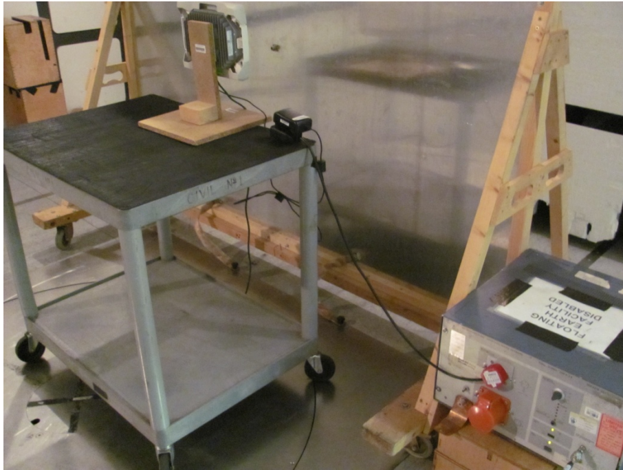
Conducted Emissions ACDC 12V Adaptor
