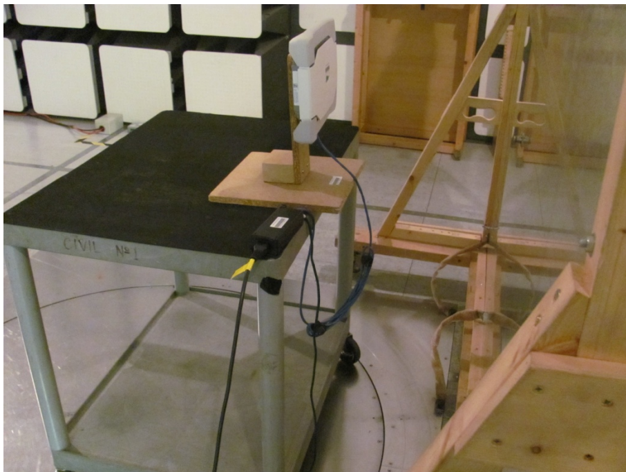
Conducted Emissions POE Inserter Microsemi
