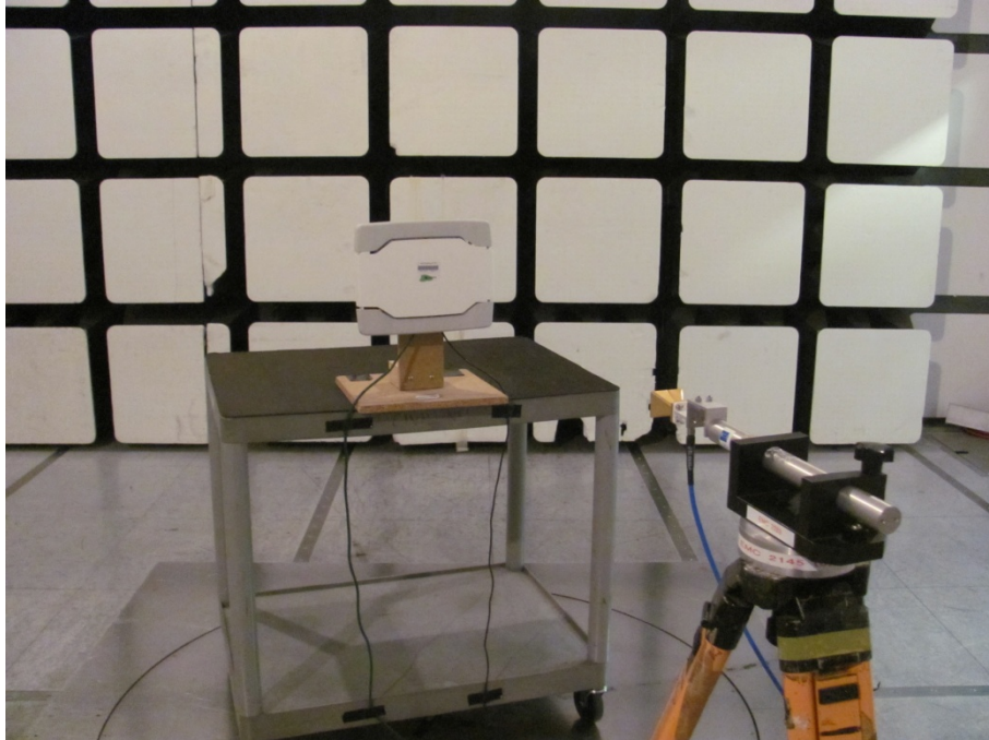
Radiated Emissions 18-20GHz
