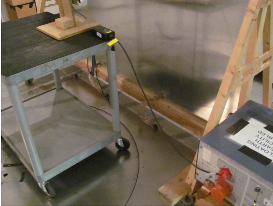
Conducted Emissions POE Inserter Phihong
