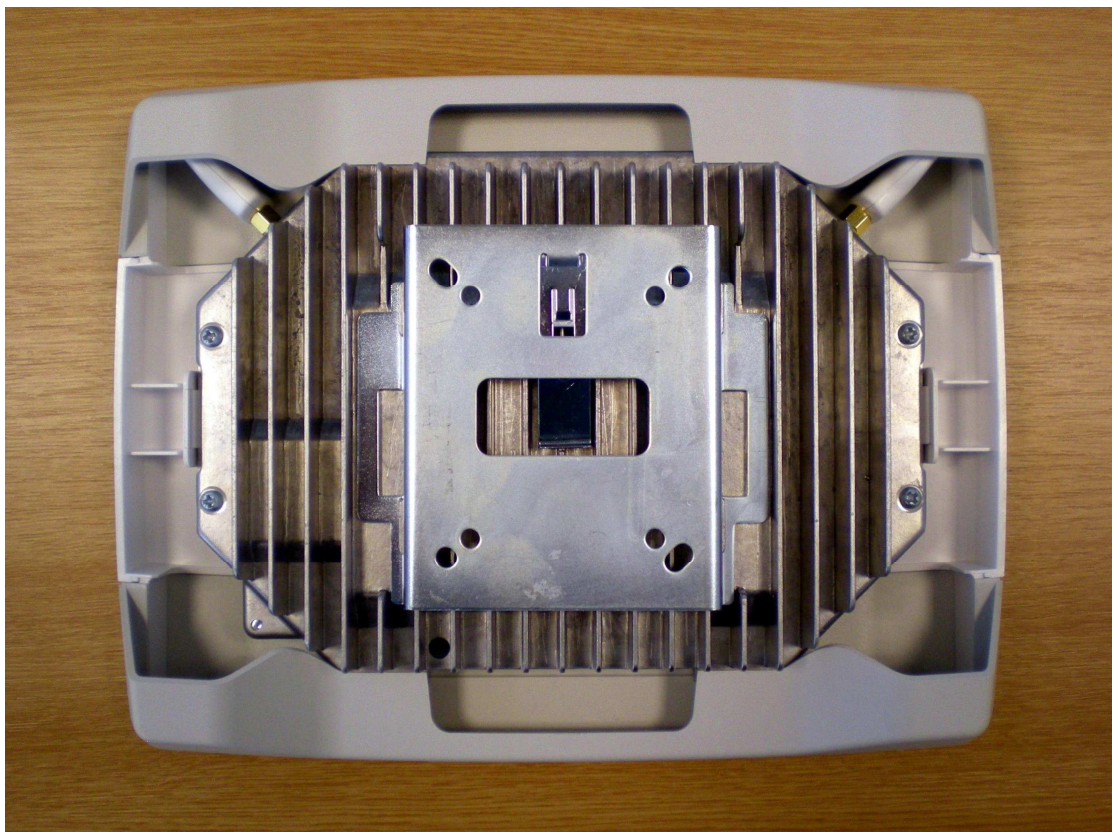
217 – Back View
