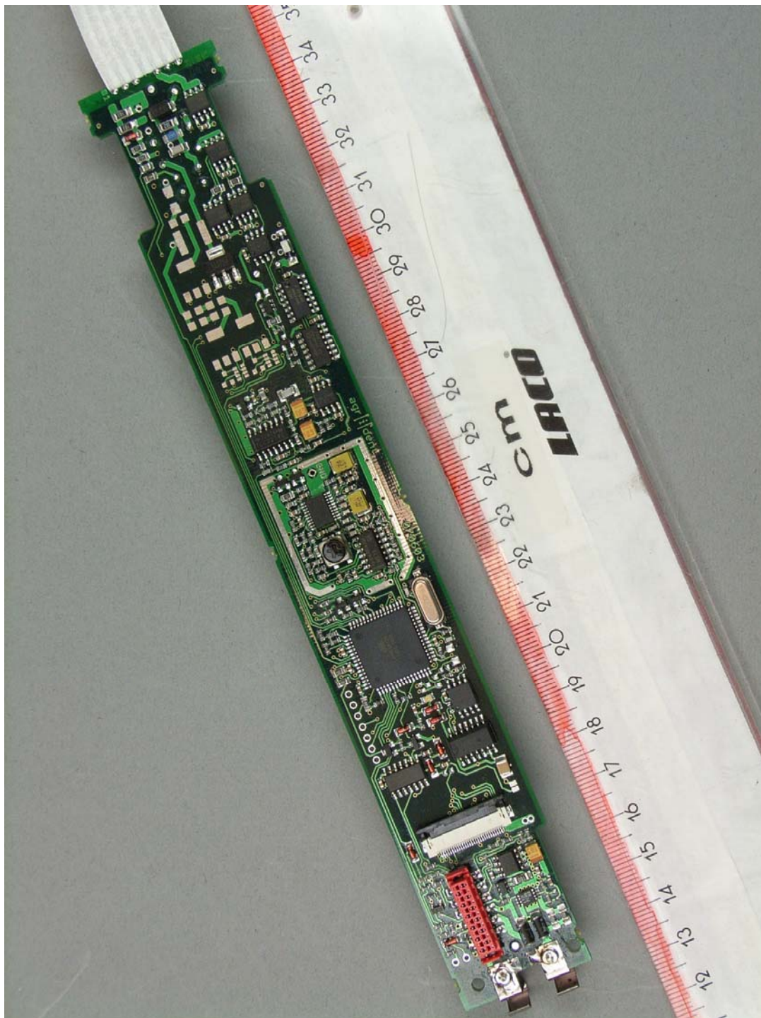
71641_15.jpg AWR100, main PCB, top view
