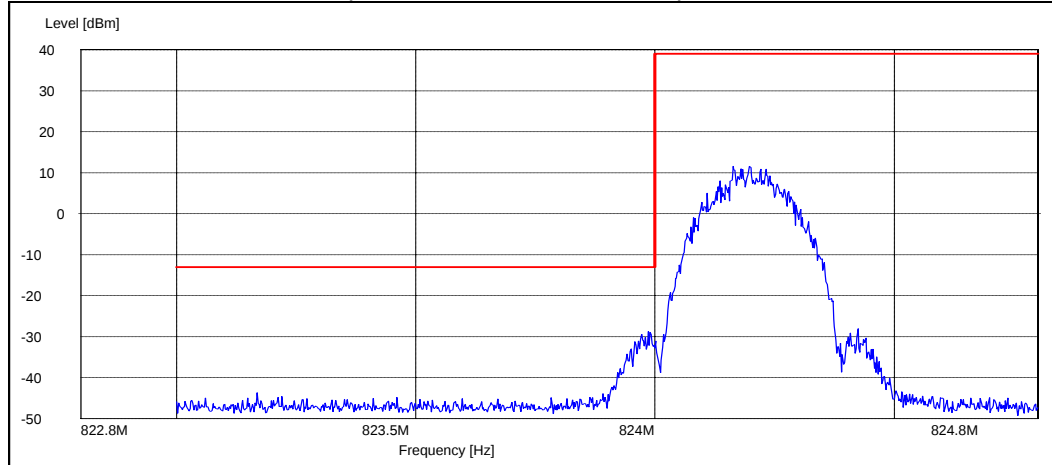
EGPRS mode, channel 128 (Peak detector, RBW: 3 kHz)
