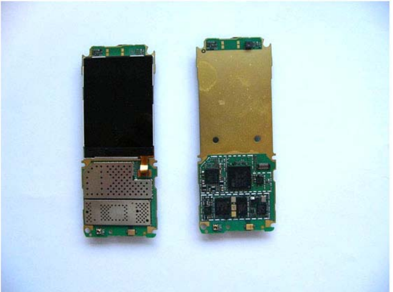
PWB front
