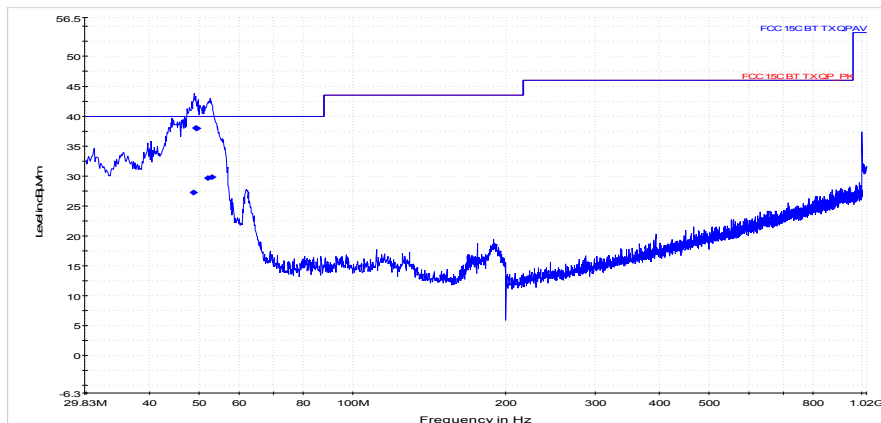
Radiated Emissions 30-1000 MHz
