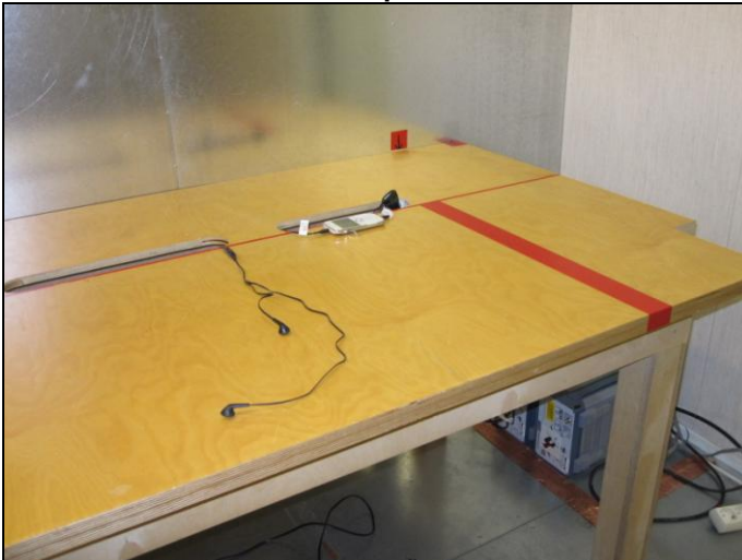
Picture 2. FCC Part 15C AC powerline conducted emissions
