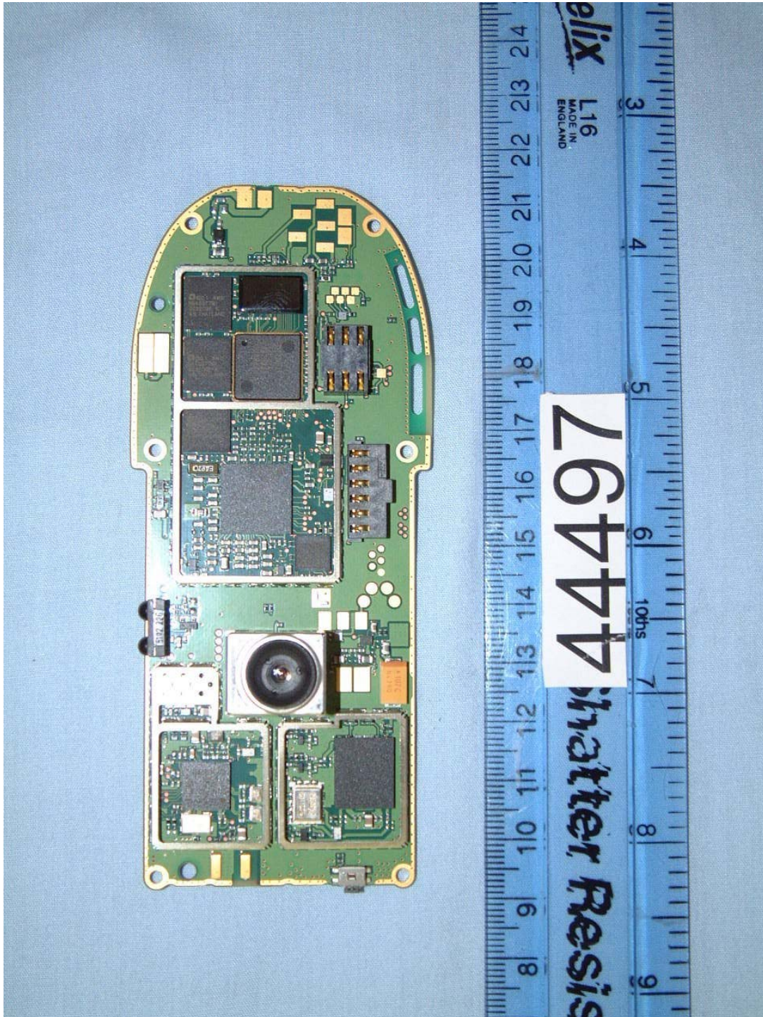
PHT\44497JD02\008 Top view of Circuit Board
