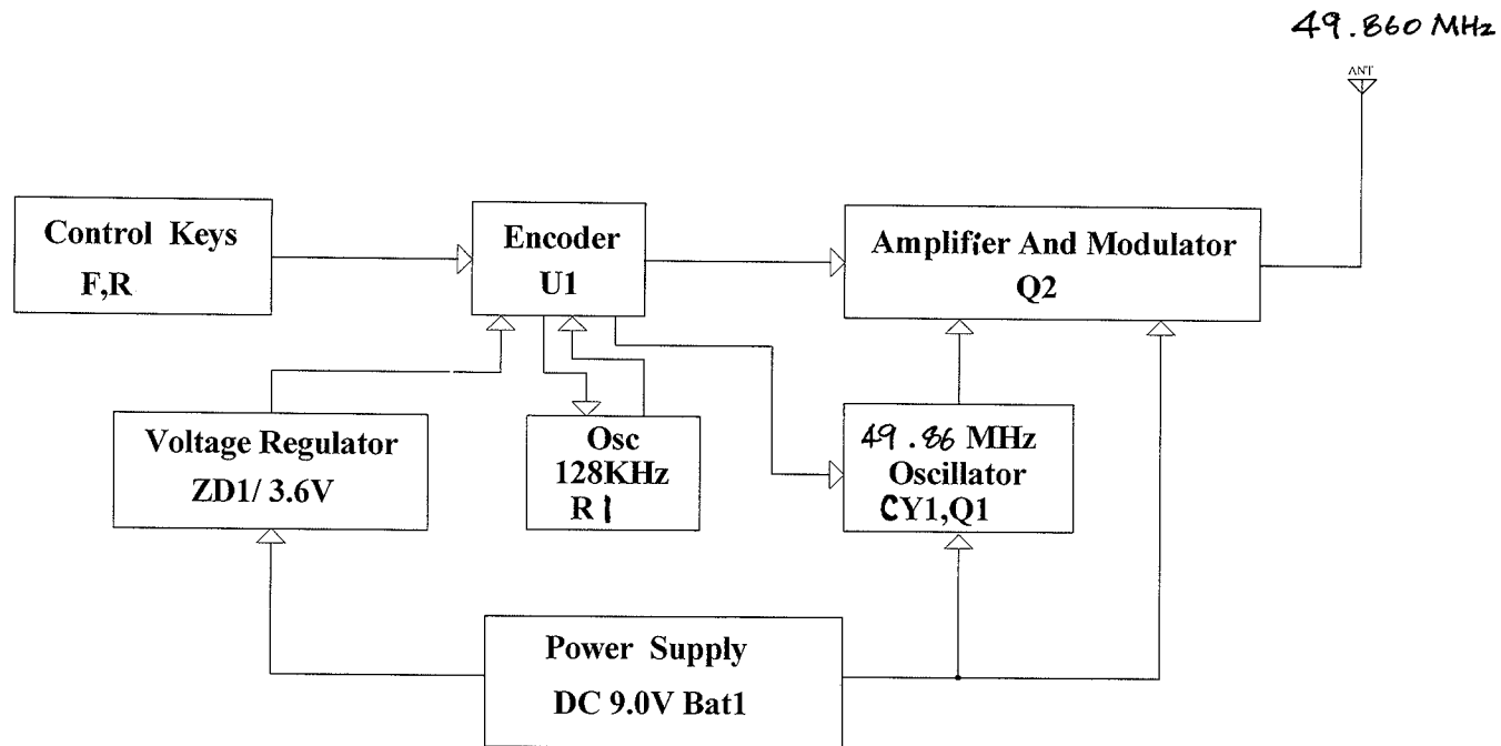
TX-49.860MHz FUNCTION BLOCK DIAGRAM
