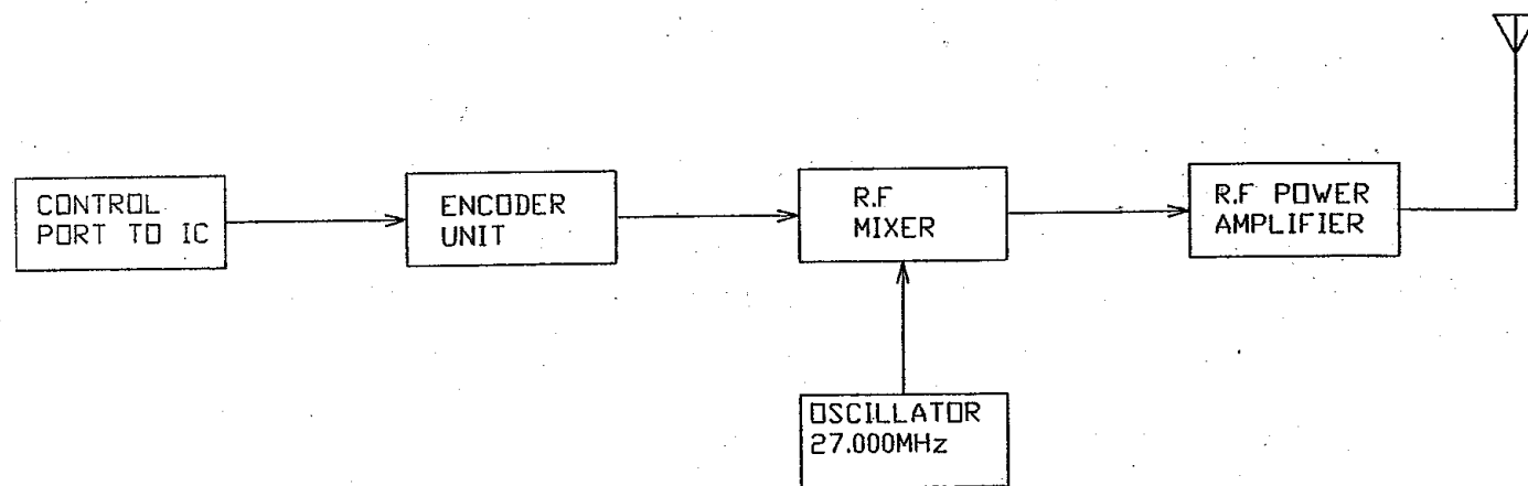
FUNCTION BLOCK DIAGRAM
