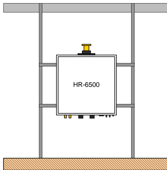
Figure 17 Suggested Mounting H-Frame
