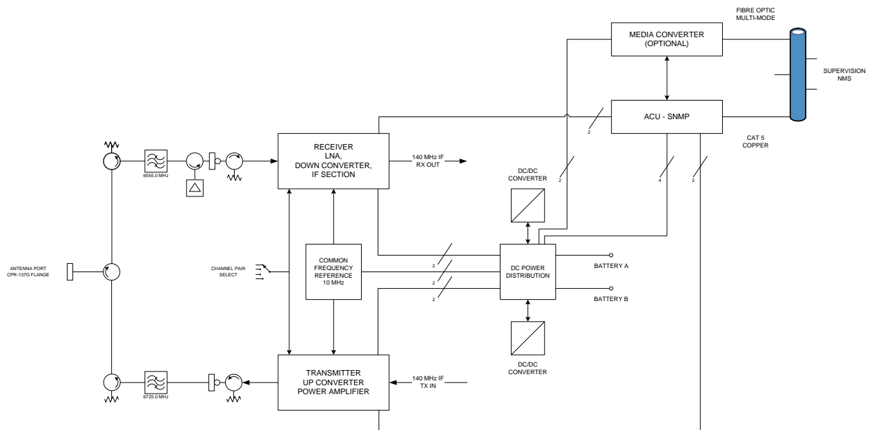
Figure 7 Block Diagram, RF Unit, 1+0 Single Channel Duplex, Equalized
