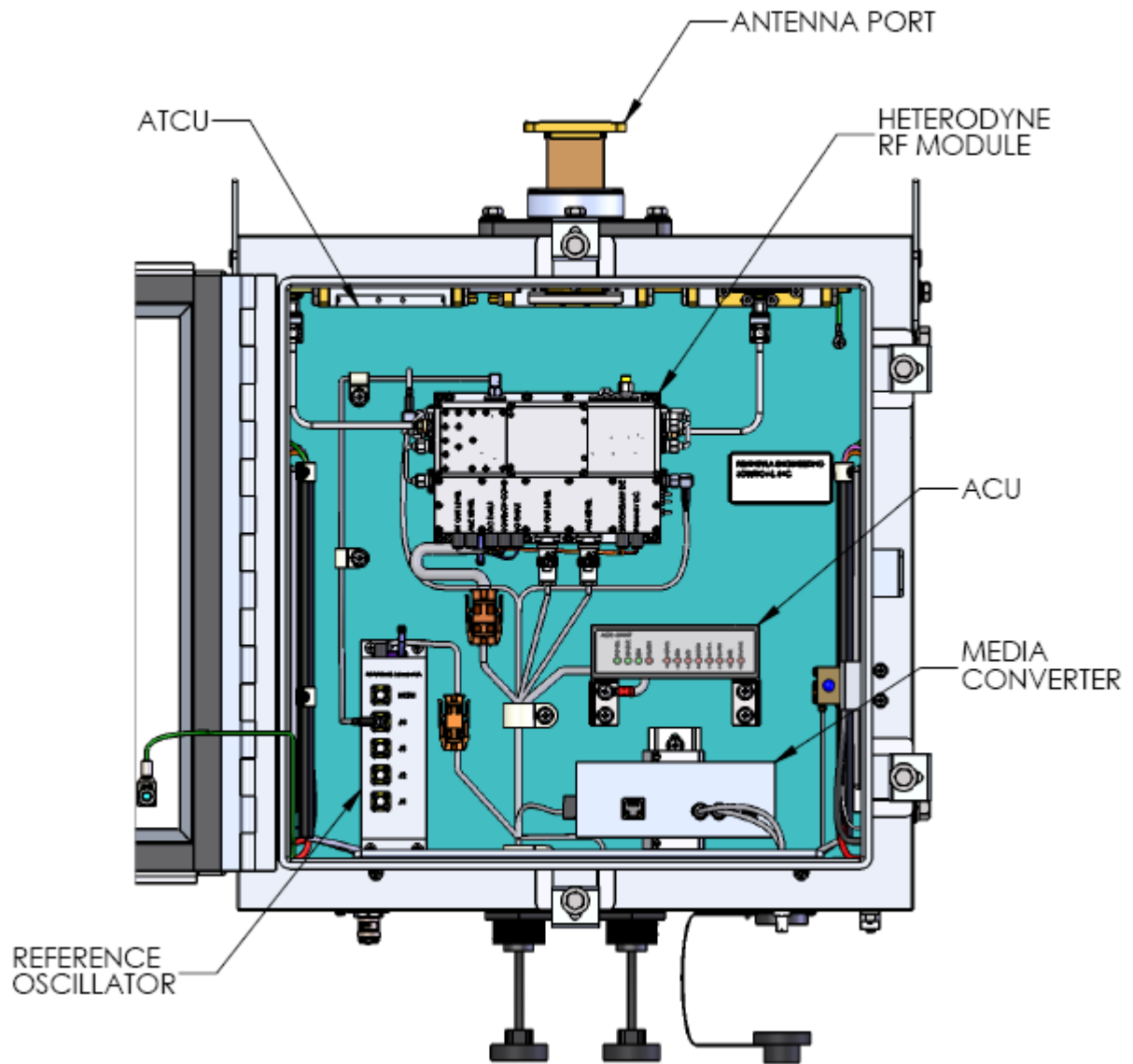
Figure 1 Mechanical Layout, HR-6500 Front View Module Locations
