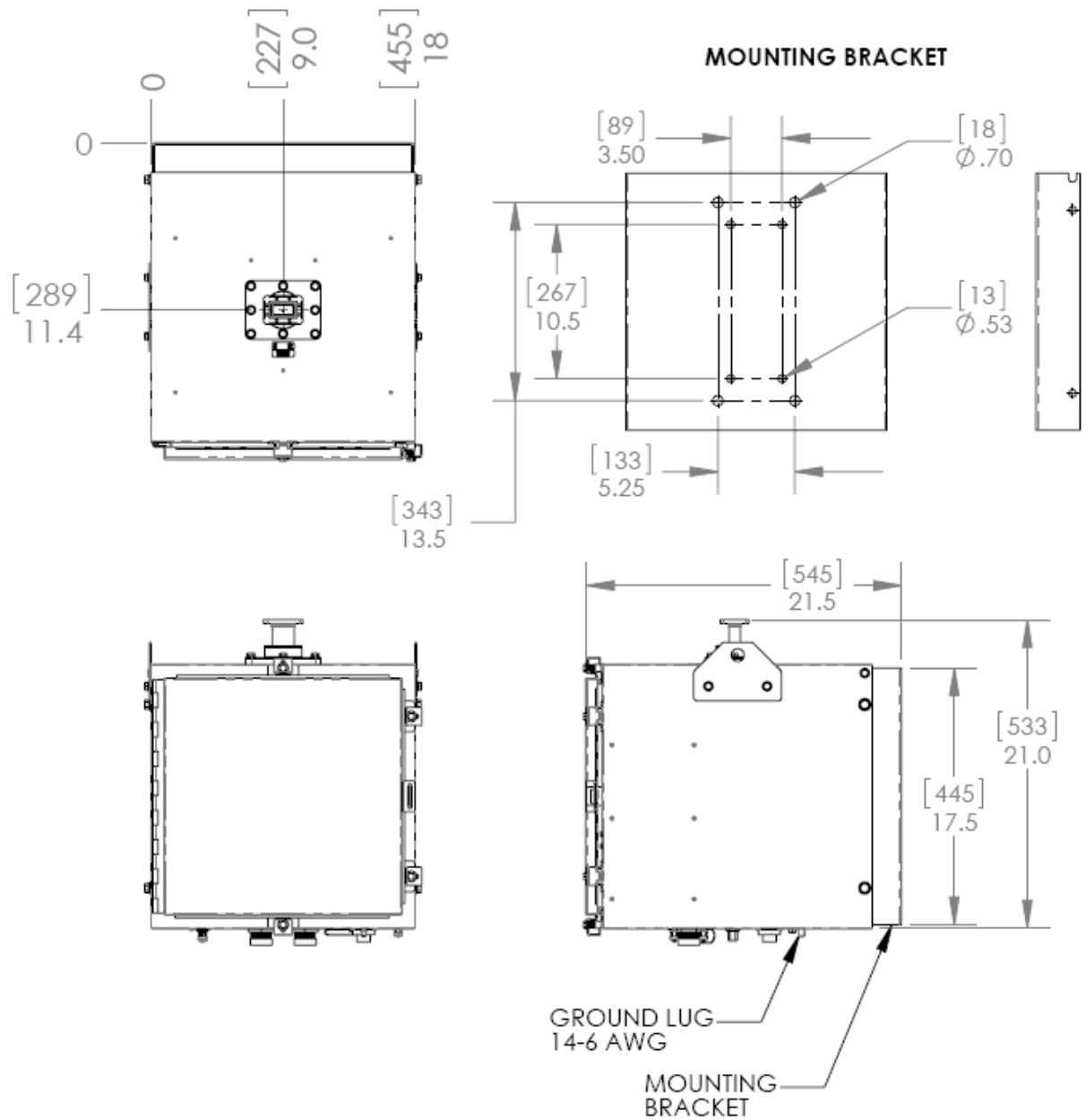
Figure 12 Enclosure Mounting Dimensions HR-6500, Single Channel Duplex
