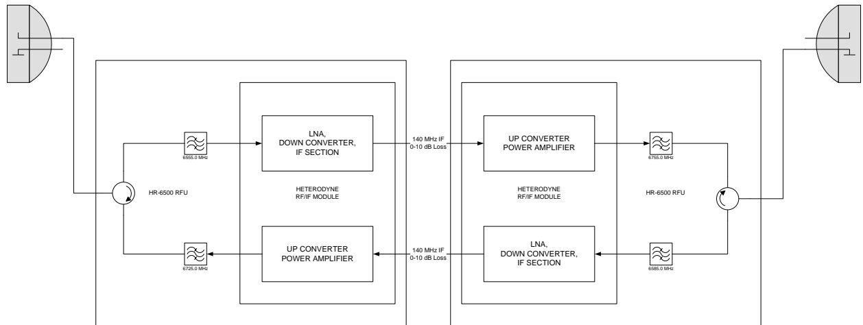
Figure 4 Block Diagram, 1+0, Heterodyne Repeater
