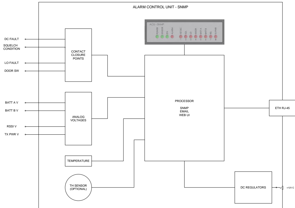
Figure 8 Block Diagram, Alarm Control Unit – SNMP
