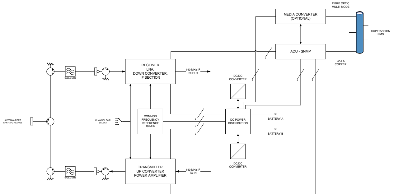
Figure 6 Block Diagram, RF Unit, 1+0 Single Channel Duplex, Un-Equalized
