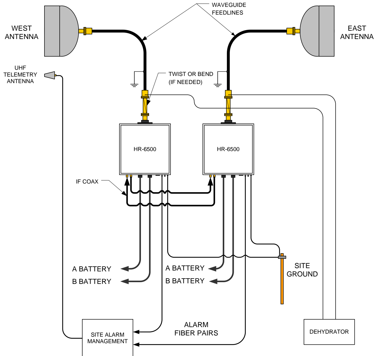
Figure 11 Typical Heterodyne Repeater Station Installation
