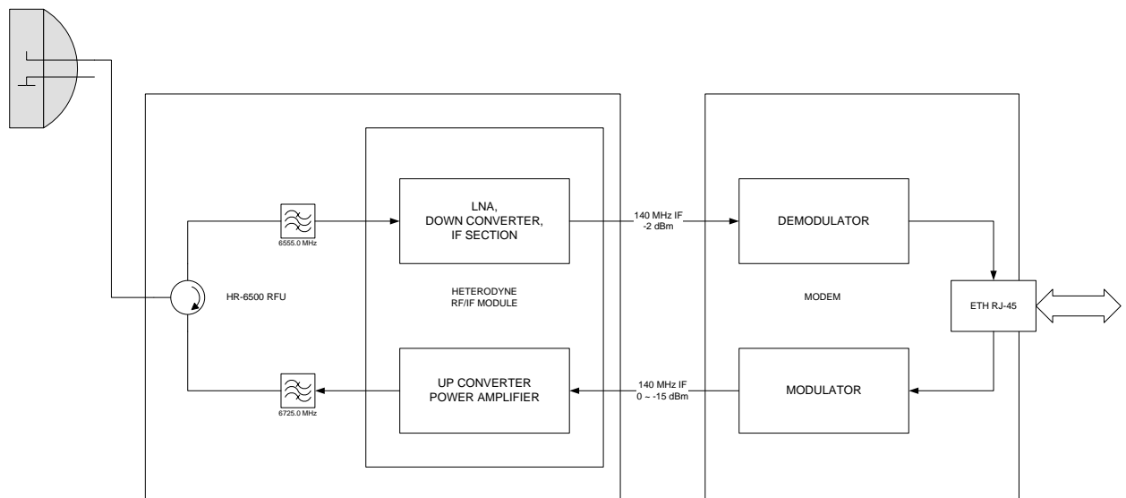
Figure 5 Block Diagram, 1+0, Heterodyne Terminal with External Modem
