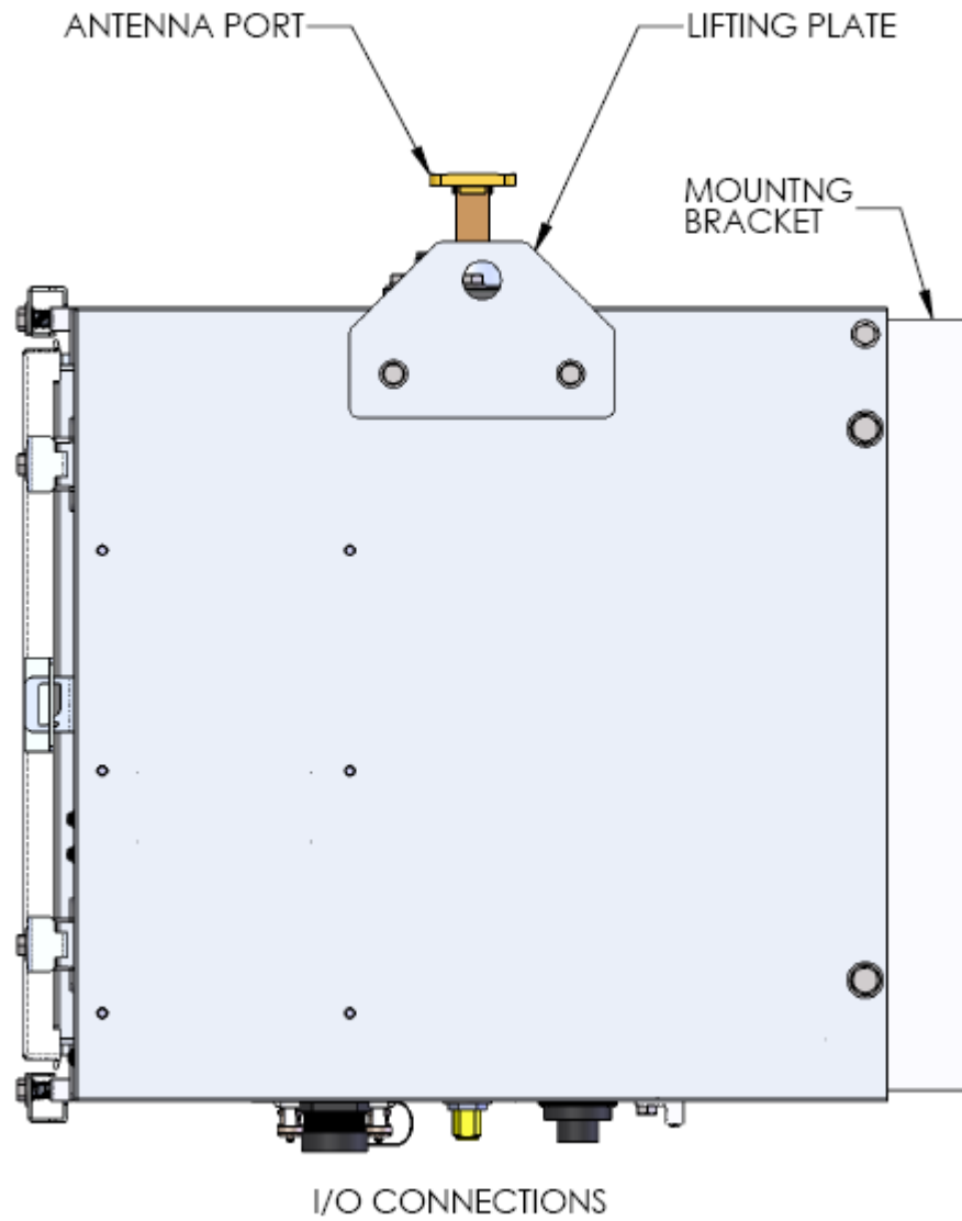
Figure 2 Mechanical Layout, HR-6500 Side View
