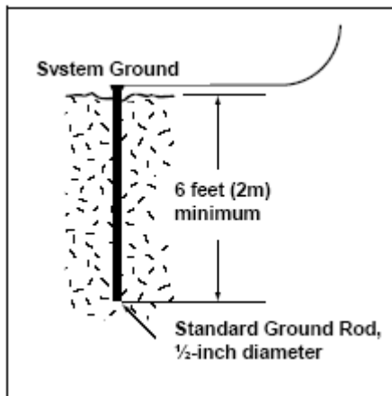
Figure 19 Typical System Ground Rod
