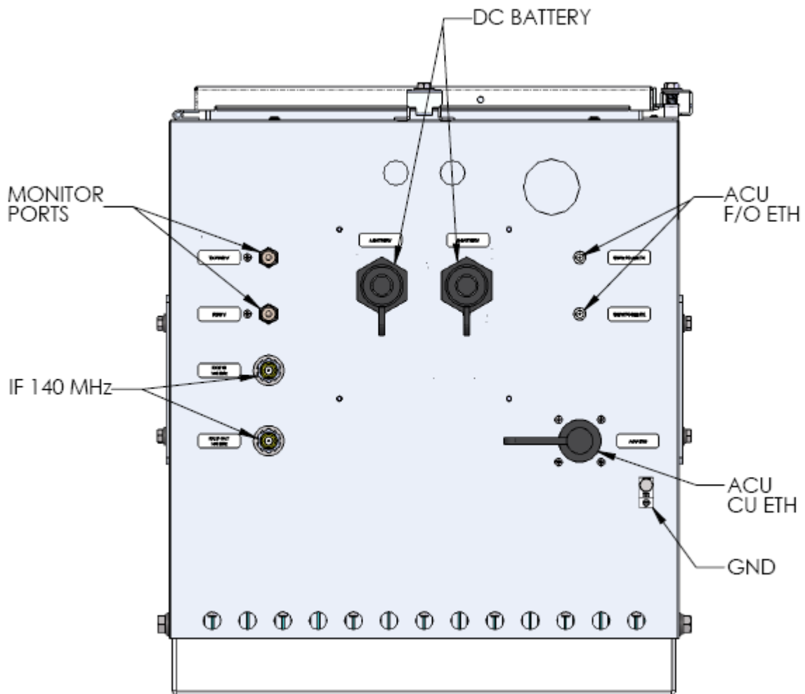
Figure 3 Mechanical Layout, HR-6500 Bottom View I/O Connections
