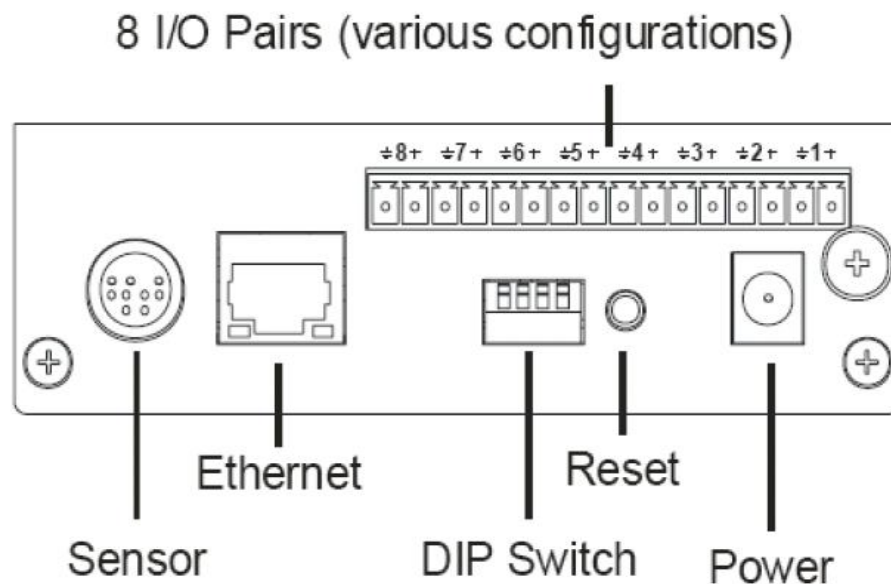
Figure 39 ACU Rear Panel
