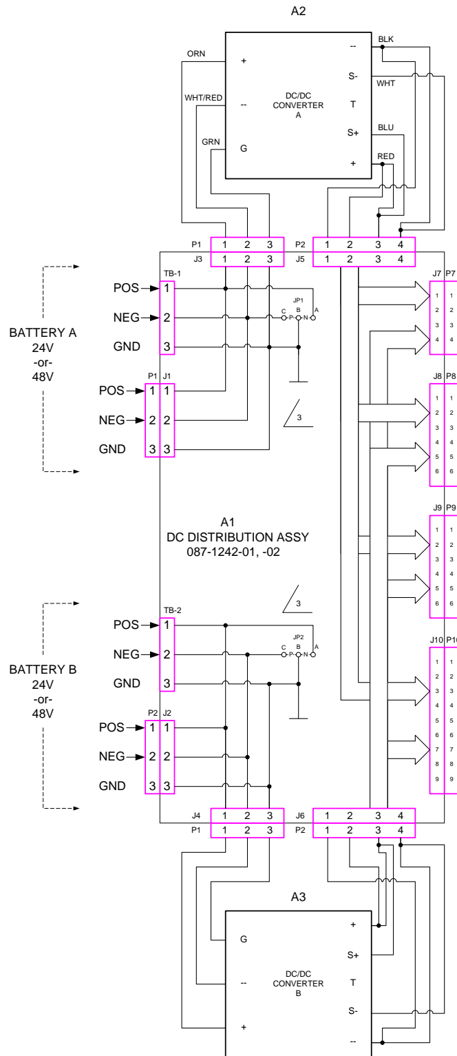
Figure 10 DC Power Connection Diagram, 24V or 48V
