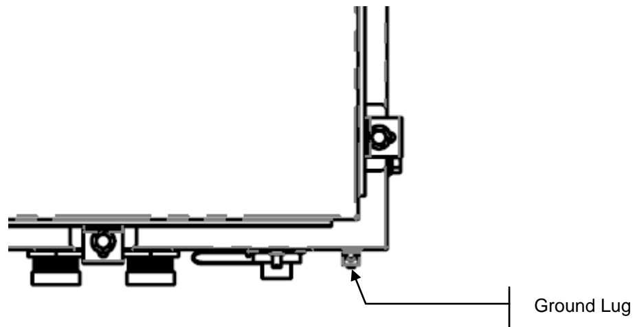
Figure 18 Location of Ground Lug on Heterodyne Repeater Enclosure
