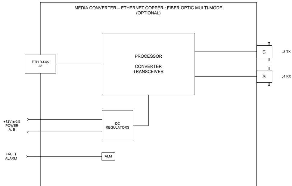
Figure 9 Media Converter, Ethernet Copper - Multi-Mode Fiber Optic
