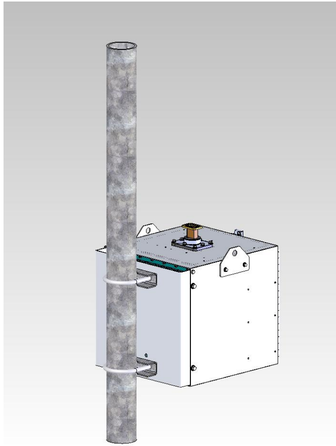
Figure 14 Heterodyne Repeater on pipe mount, rear view
