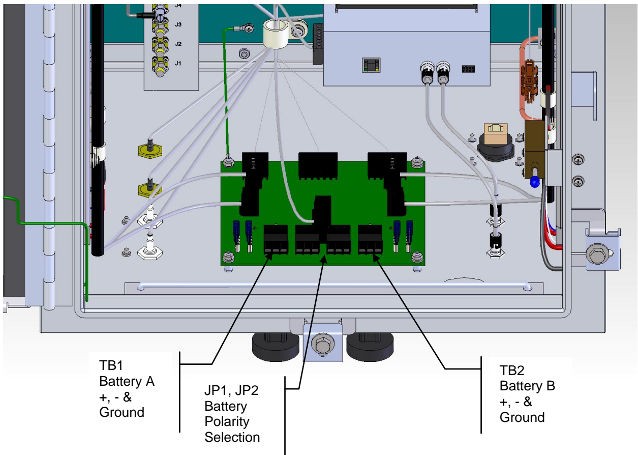
Figure 20 Wiring and Ground Connections, Power Distribution Assembly
