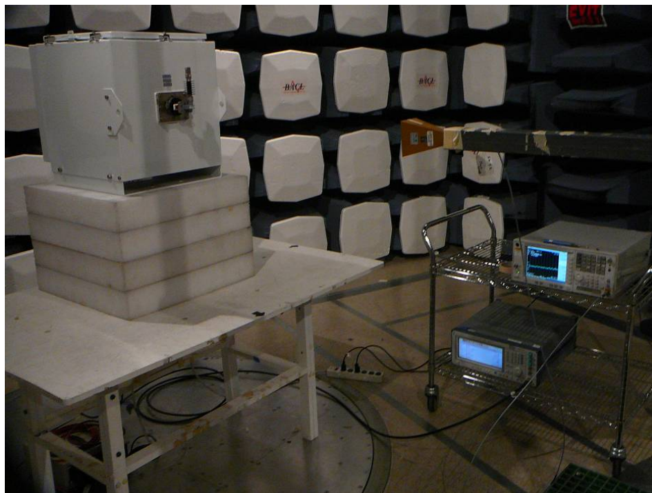
18-26 GHz Radiated Emission – View
