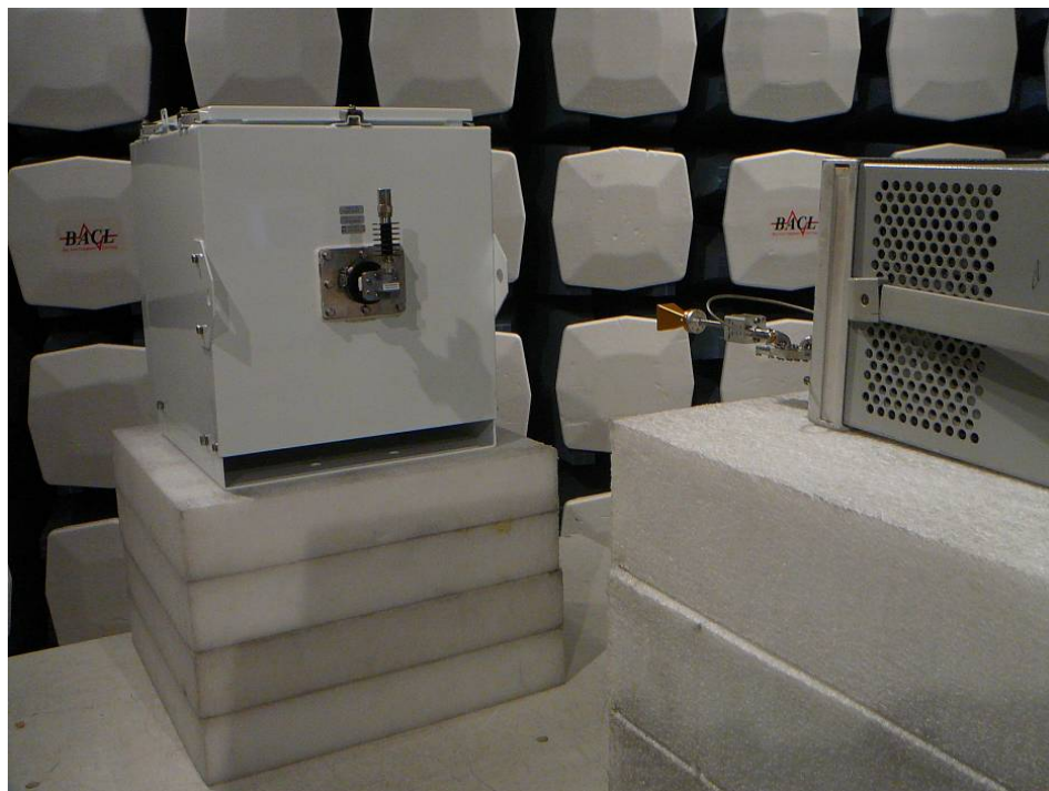
90-120 GHz Radiated Emission – Rear View
