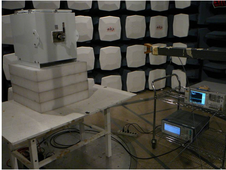
40-60 GHz Radiated Emission – View
