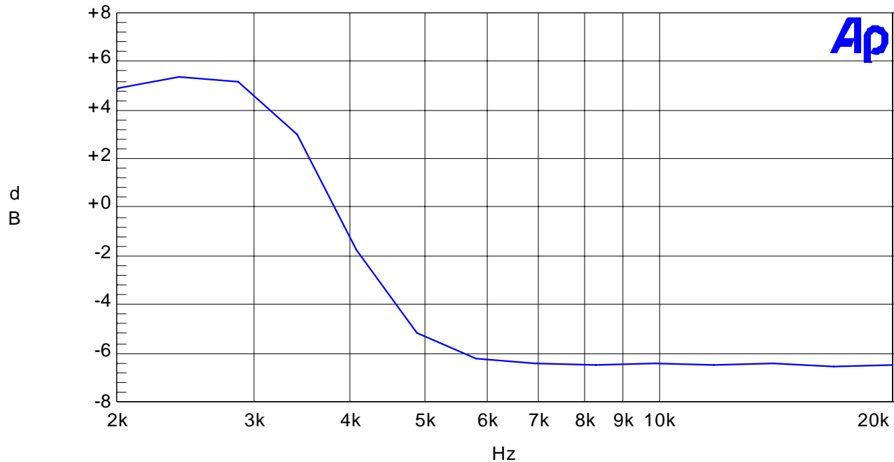
Audio Low Pass Filter
