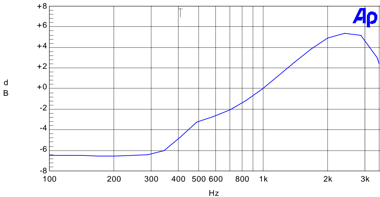
Audio Frequency Response Plot
