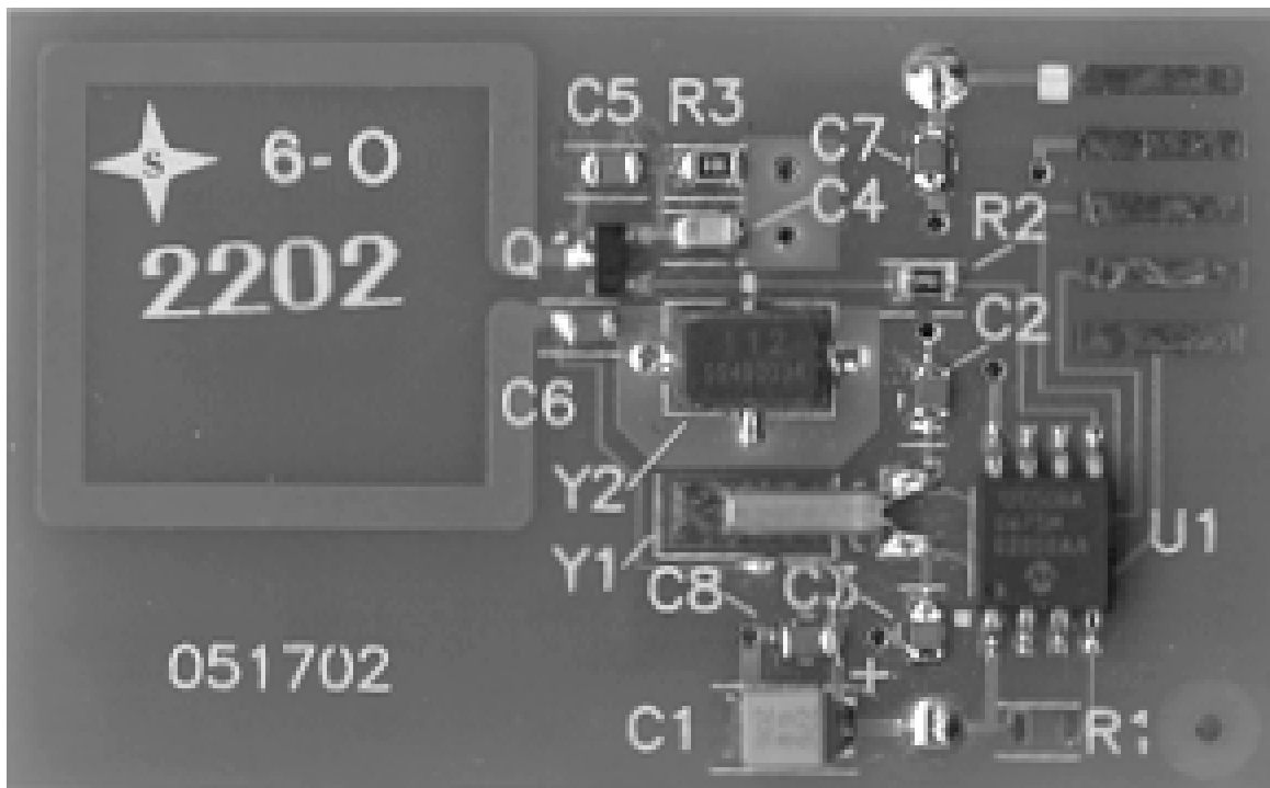
BullzI Tag, PCB Component Side, X3 Magnification
