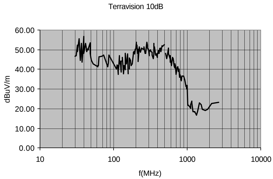
FIGURE 3.2-1 TERRAVISION 10DB BANDWIDTH
