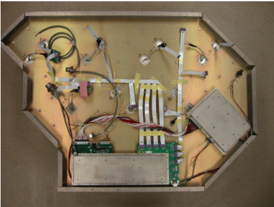
OPENED ANTENNA. SEE DOCUMENT QF7TERRAVISION ANTENNA ELECTRONICS FOR DETAILS
