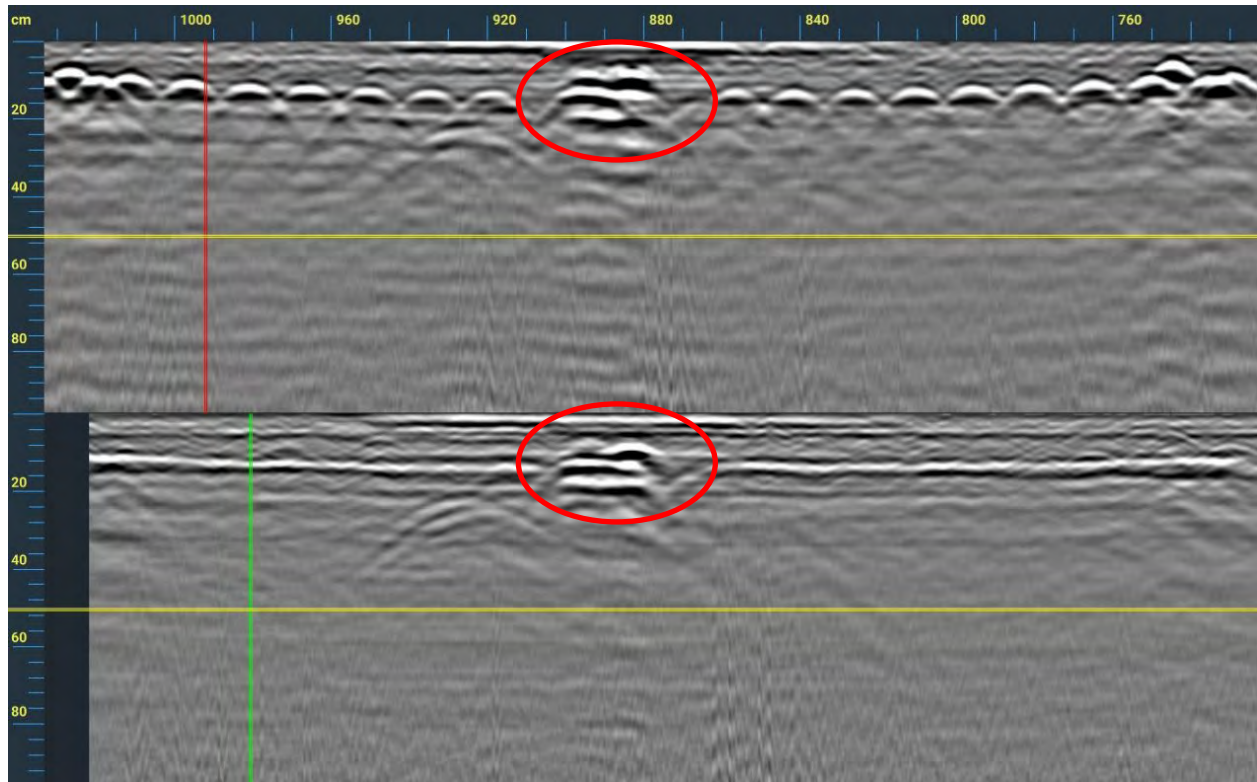
Conduit located beneath a wire mesh layer. The wire mesh hyperbolas disappear in the cross-polarized data, becoming a coherent layer and further revealing the conduit beneath.
