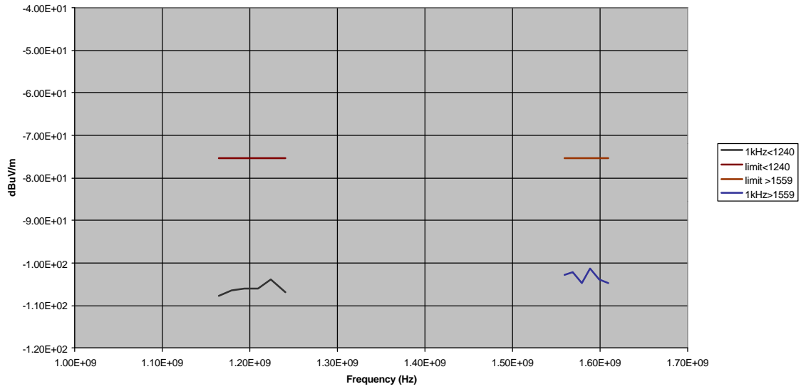
FIGURE 4.3-1 INTERRAGATOR RMS (GPS; RBW=1kHz)
