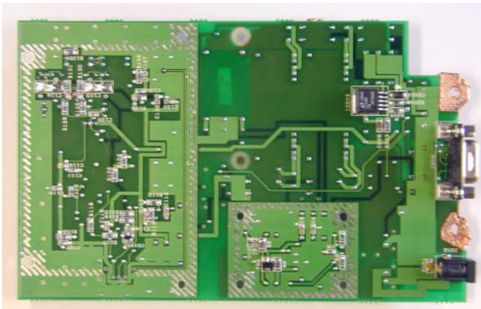
Transmitter-Receiver Circuit - Back
