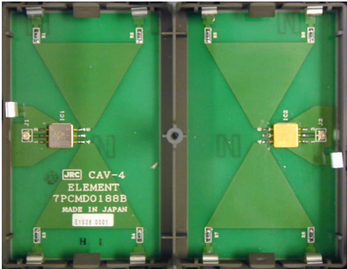
Elenent Circuit (Transmitter & Receiver fans)
