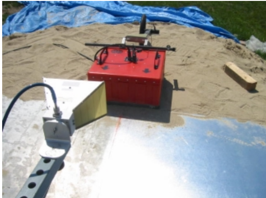
Worst-Case Radiated Emission Above 960MHz
