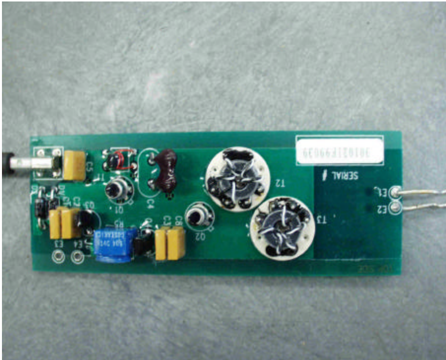
COMPONENT SIDE
