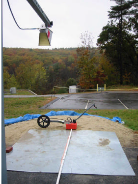
Model 5103 setup for measurements >1\text{GHz} (2.5 - 4m antenna height)
