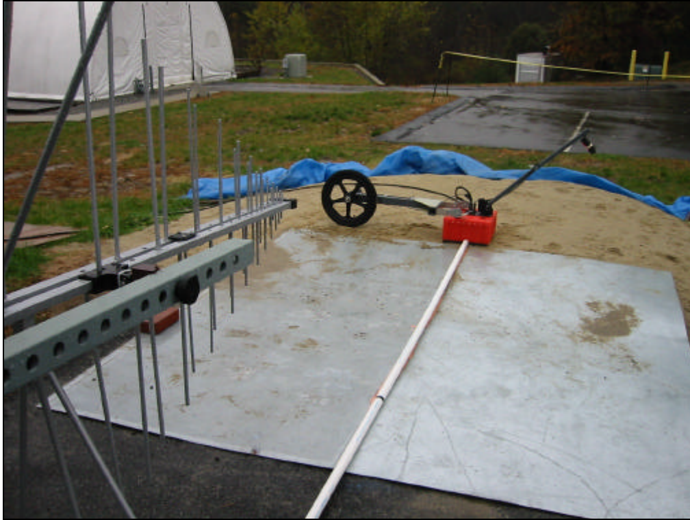
Model 5103 worst case setup for measurements <1\text{GHz}
