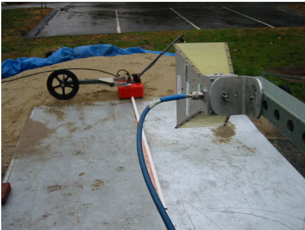
Model 5103 worst case setup for measurements >1\text{GHz} (1-2.5m antenna height)
