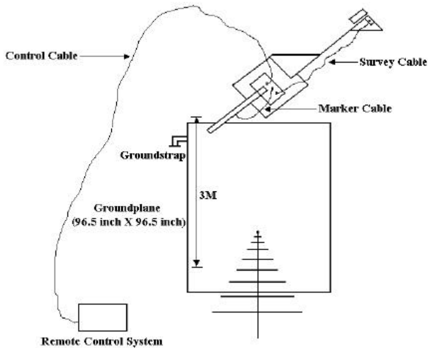
FIGURE 1-1 TEST SETUP BLOCK DIAGRAM
