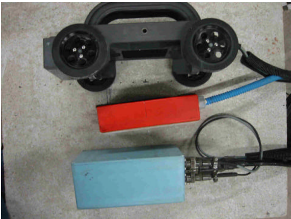
DISASSEMBLED UNIT. CART WITH ANTENNA REMOVED AND ELECTRONICS BOX WITH POUCH REMOVED.
