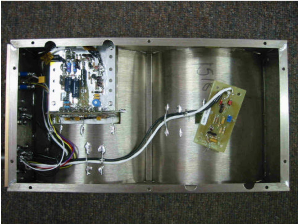
TOP VIEW OF ASSEMBLY WITH BOARD REMOVED FROM SLOT
