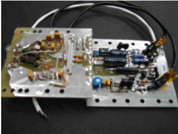
Topside shown, board is bent after Inserting into shield slot.
