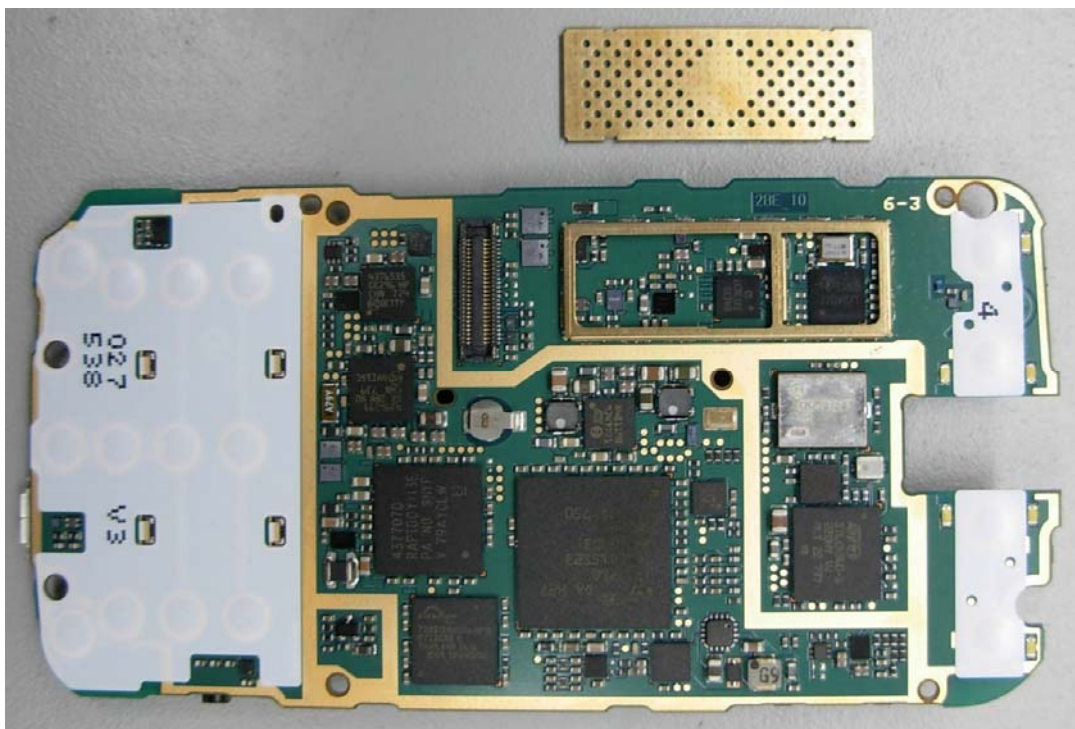
Fig 4 – PWB Front View: Shield removed
