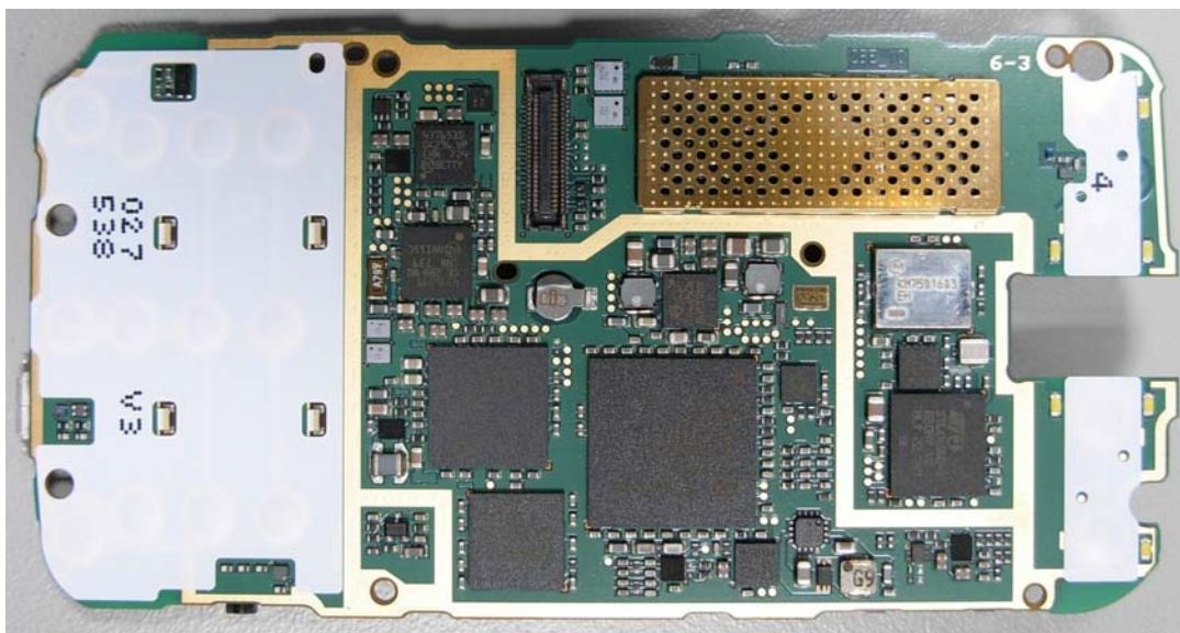
Fig 3 – PWB Front View: Shield in place
