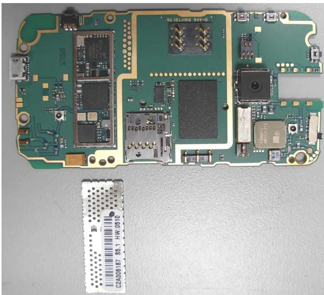
Fig 2 – PWB Back View: Shield removed
