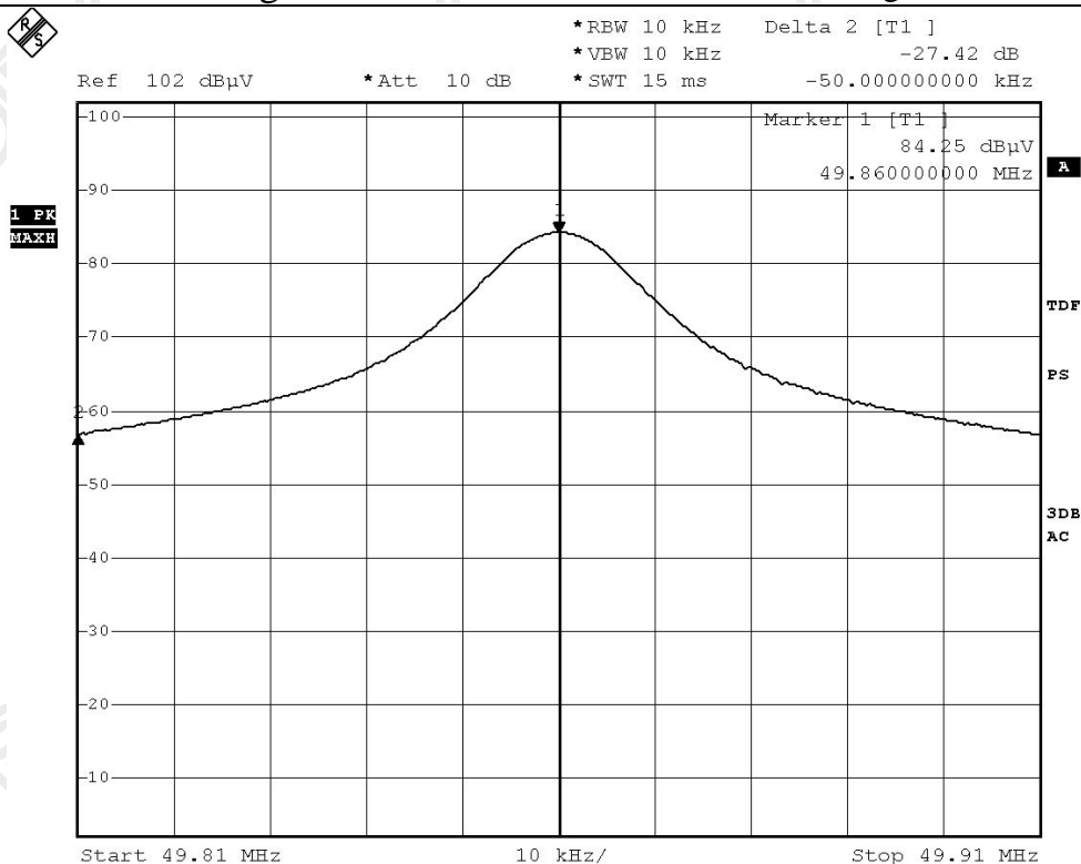
Figure D [27dB Level Reduction at Band Edge]
