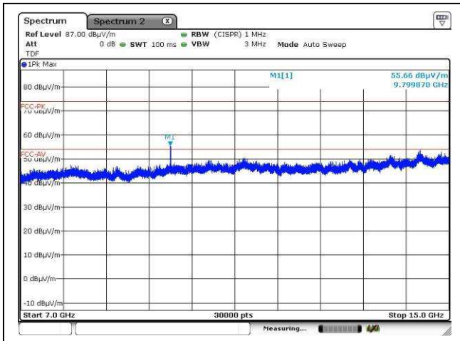
Middle channel, 7GHz – 15GHz, Horizontal
