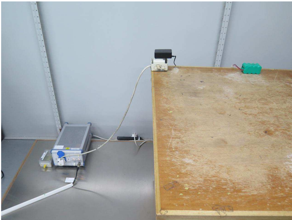
Line-conducted emission (front view, charging)
