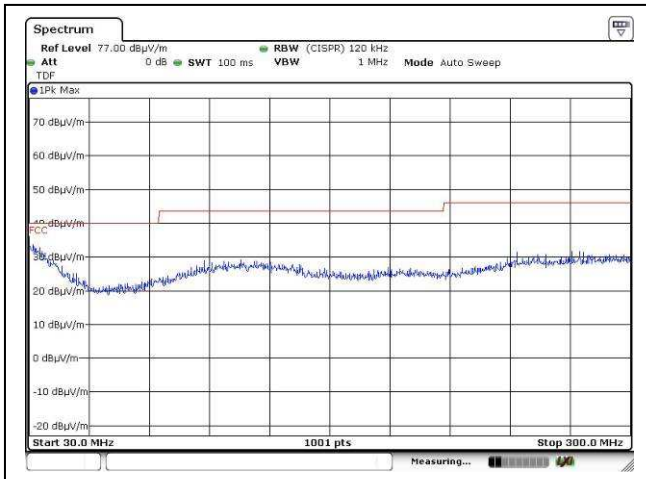
Receiving mode, 30MHz – 300MHz, Horizontal
