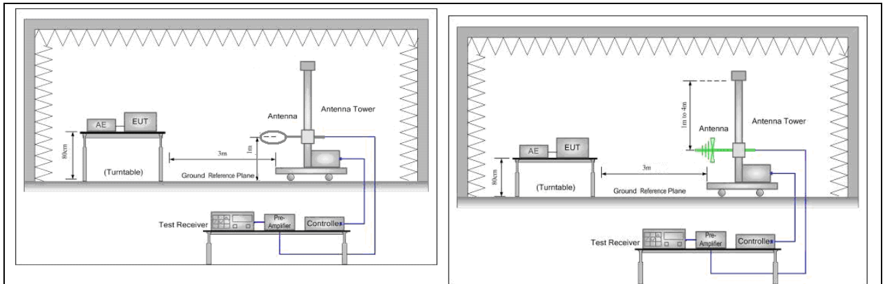
Figure 1. Below 30MHz
