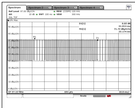
Duty Cycle 1
