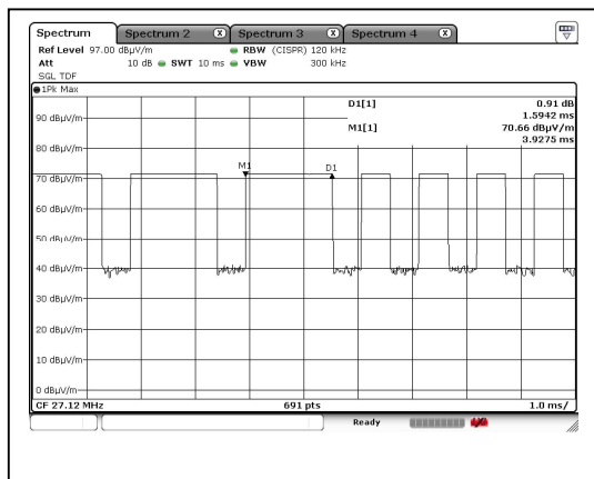
Duty Cycle 2
