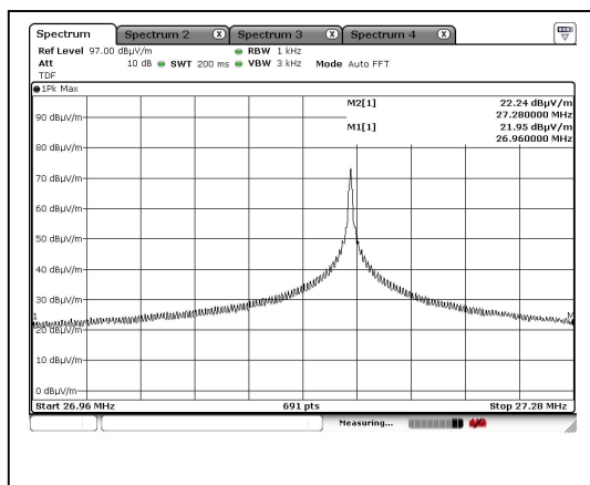
Bandwidth 1
