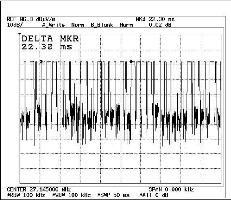
Duty Cycle
