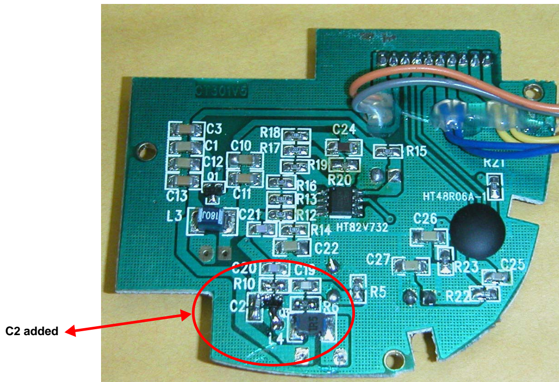
Circuit Board – top side
