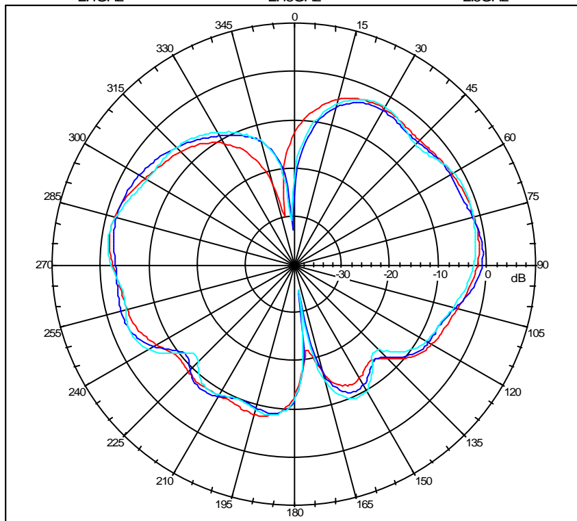
SA3 Dipole Antenna E_Plane
