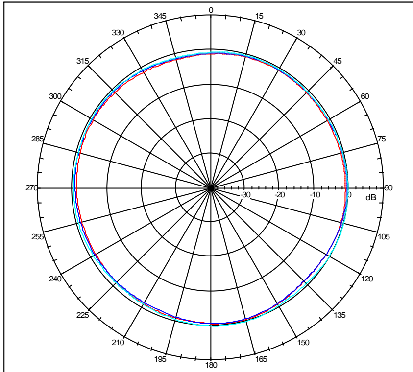
SA3 Dipole Antenna H_Plane
