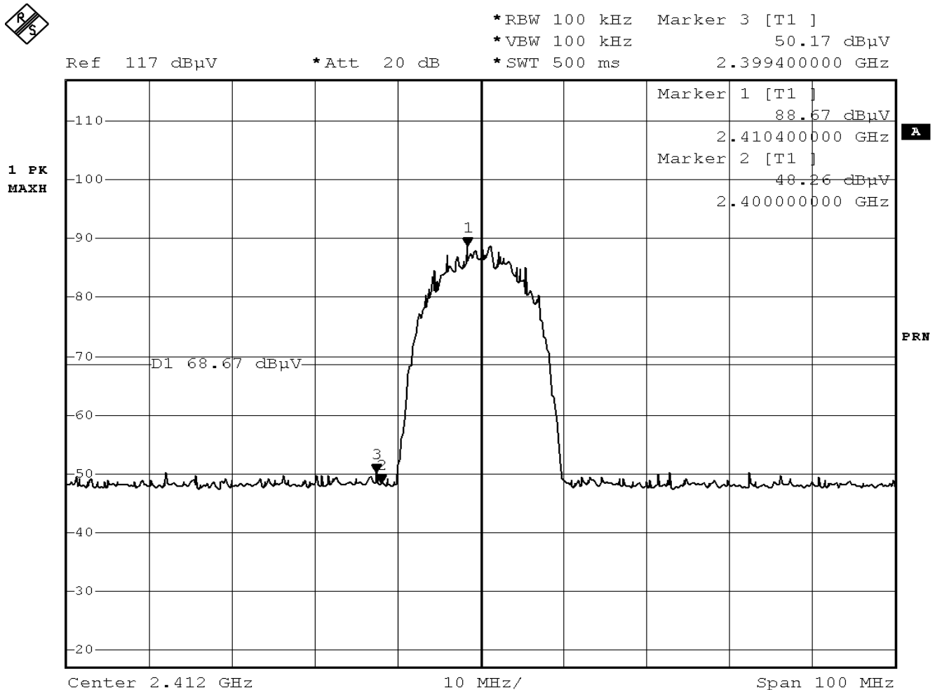
Figure Channel 1: (Horizontal)
