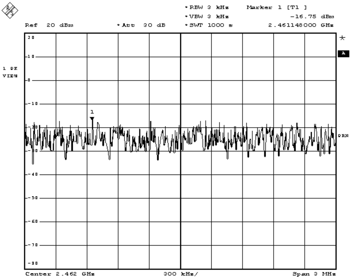
Figure Channel 11: 11Mbps
