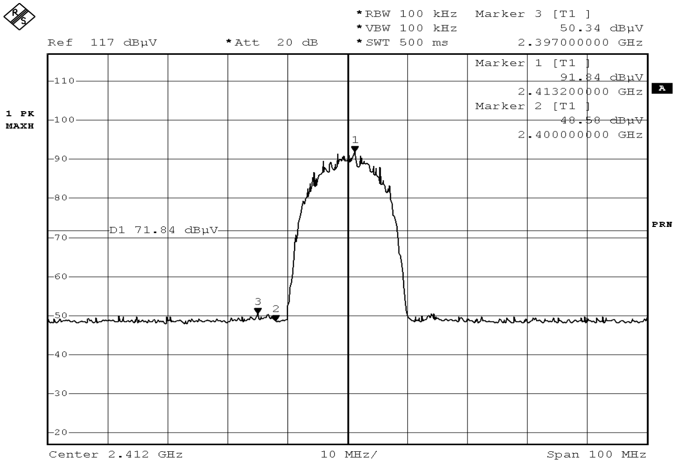
Figure Channel 1: (Vertical)
