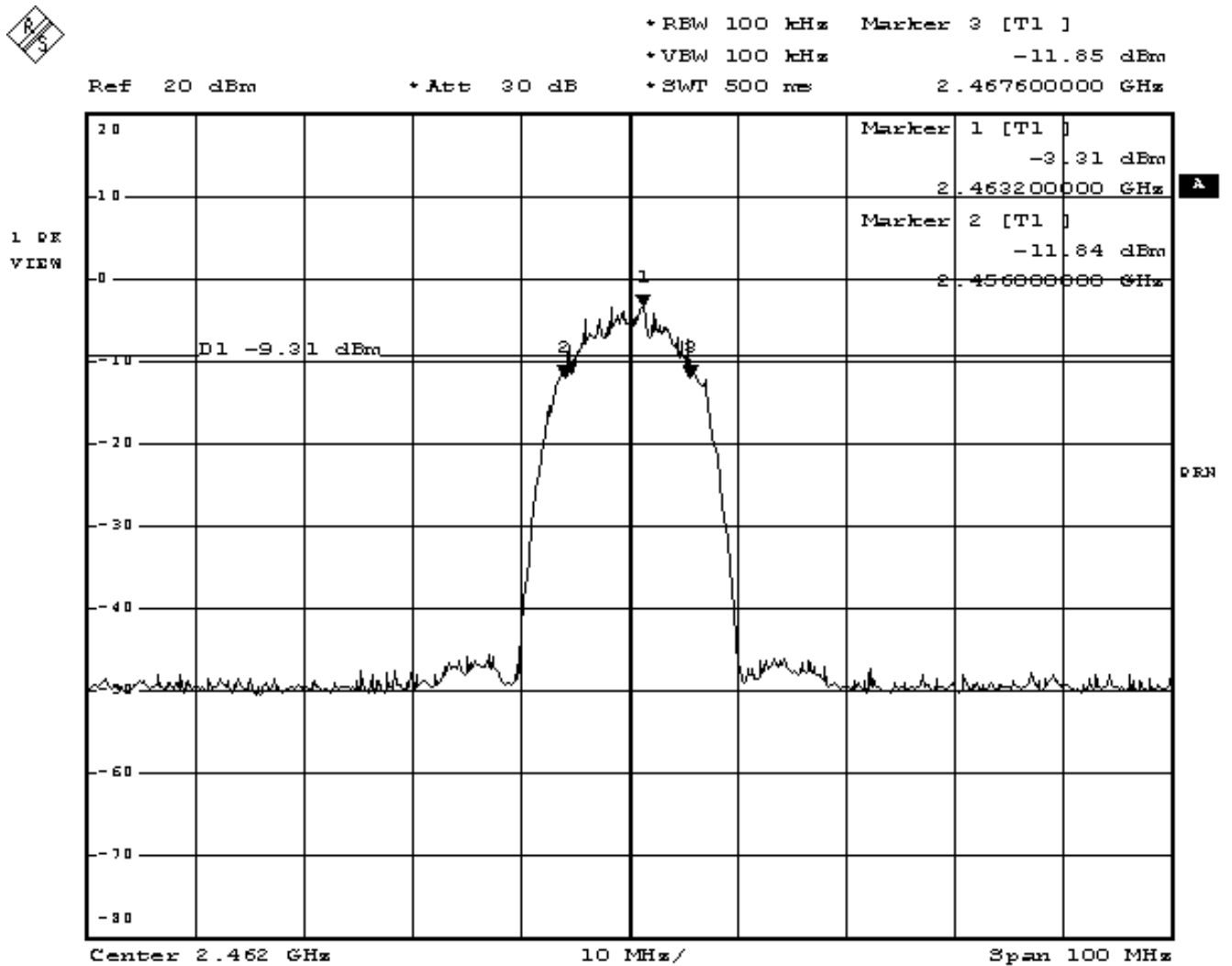
Figure Channel 11: 11Mbps
