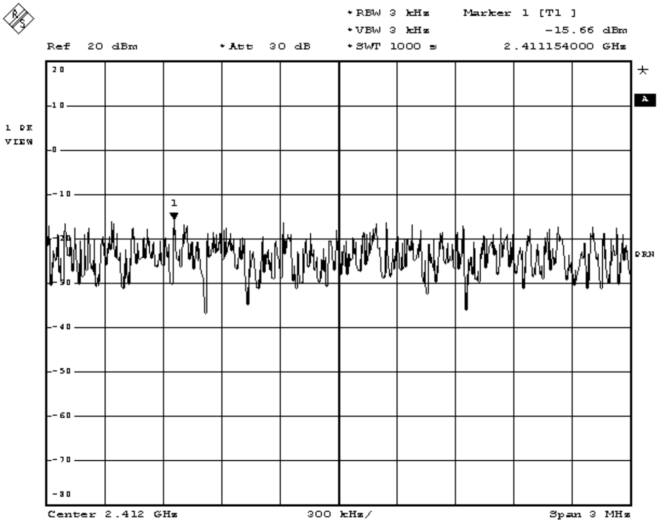
Figure Channel 1: 11Mbps
